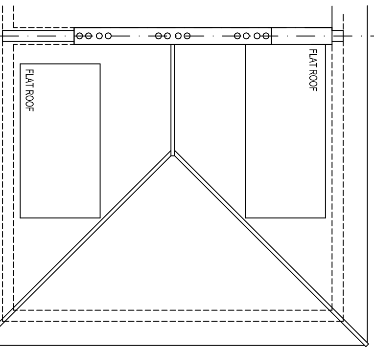
ROOF PLAN
