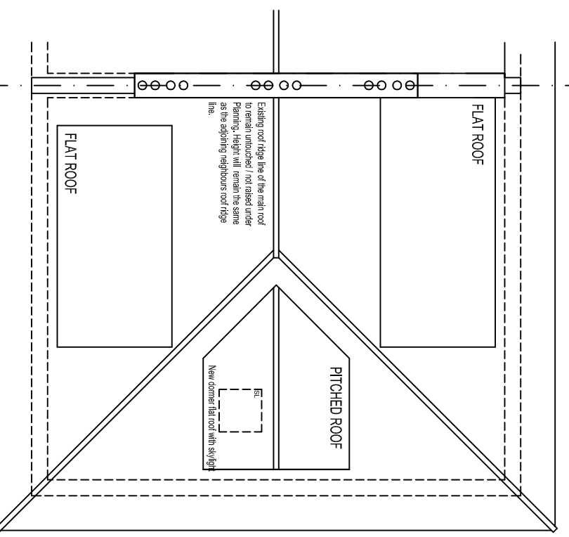
ROOF PLAN
