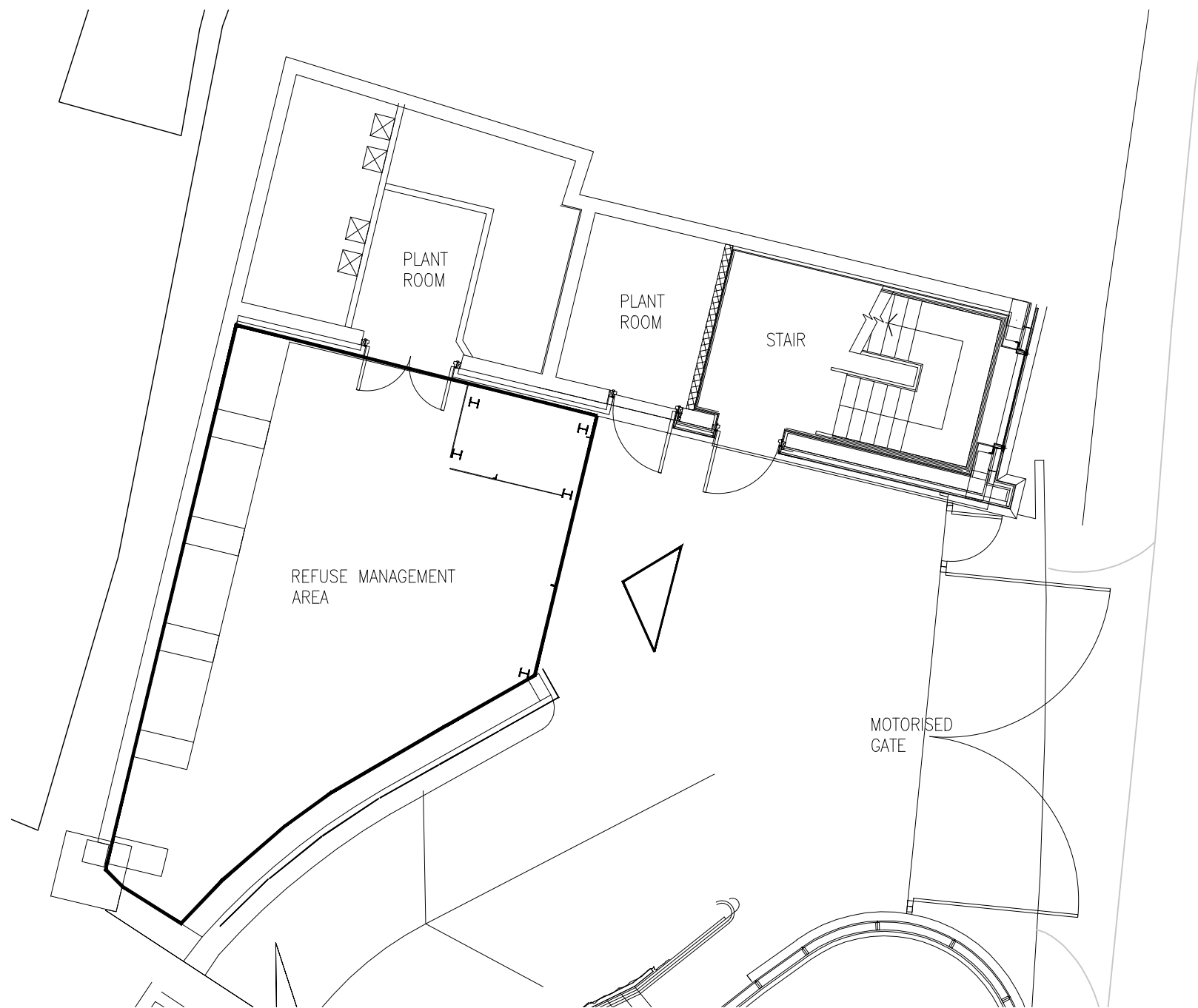
1 LOWER GROUND FLOOR PLAN SCALE 1:100
