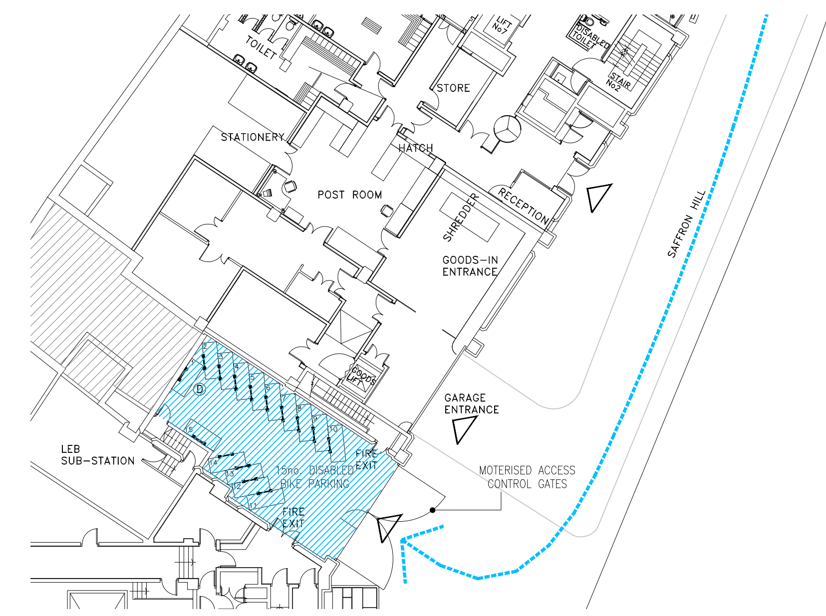
1 LOWER GROUND LEVEL PLAN - CYCLE PARKING SCALE 1:200
