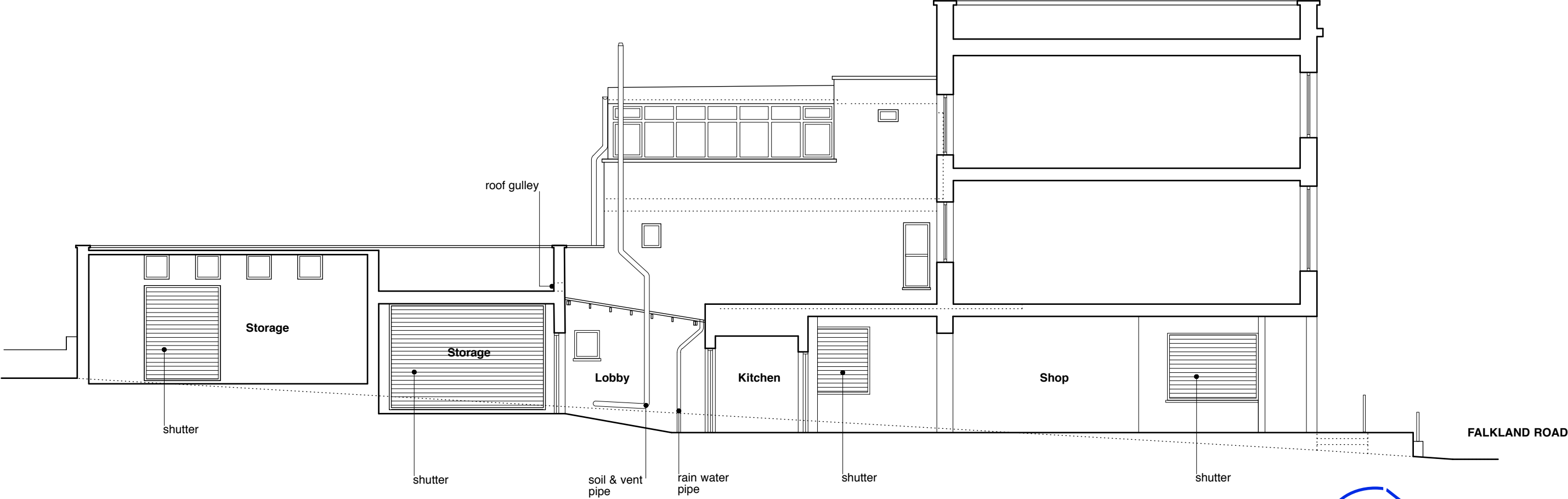
EXISTING SECTION AA scale 1:100
