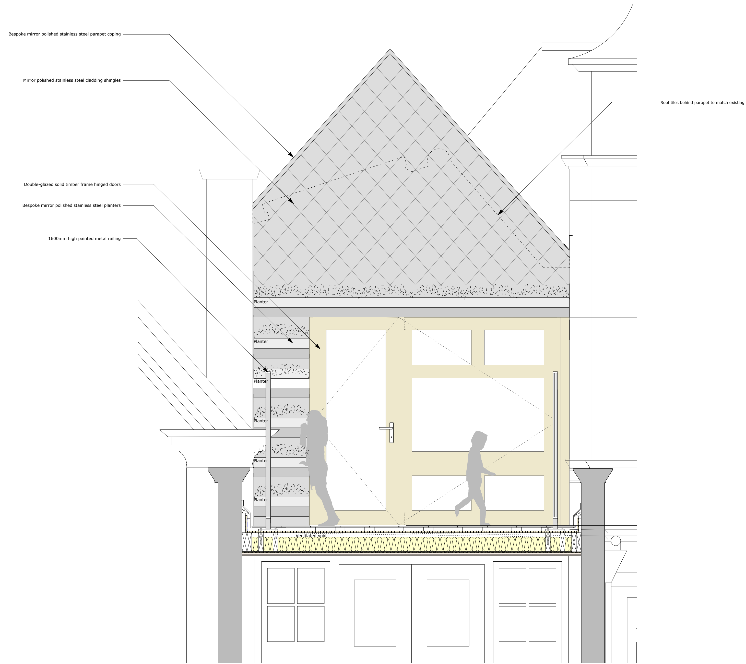
Rooftop Extension Elevation 1:20
