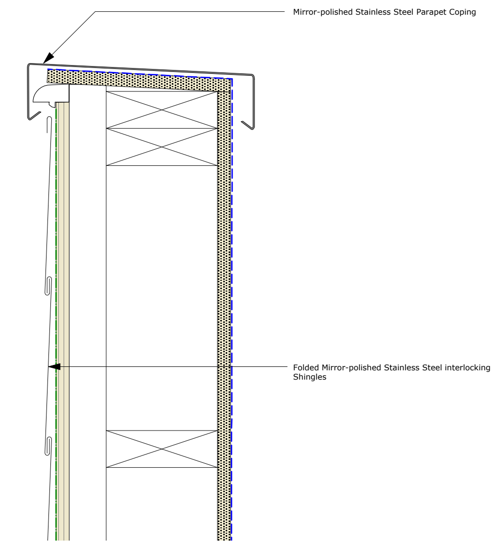
Section Detail Through Parapet 1:5
