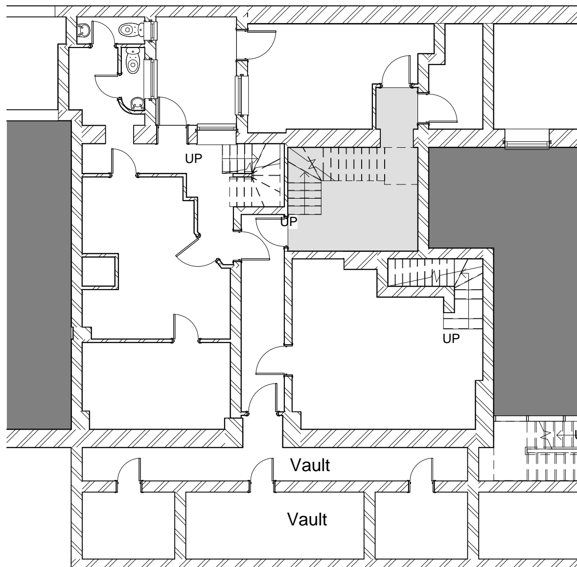
Basement 1:100
