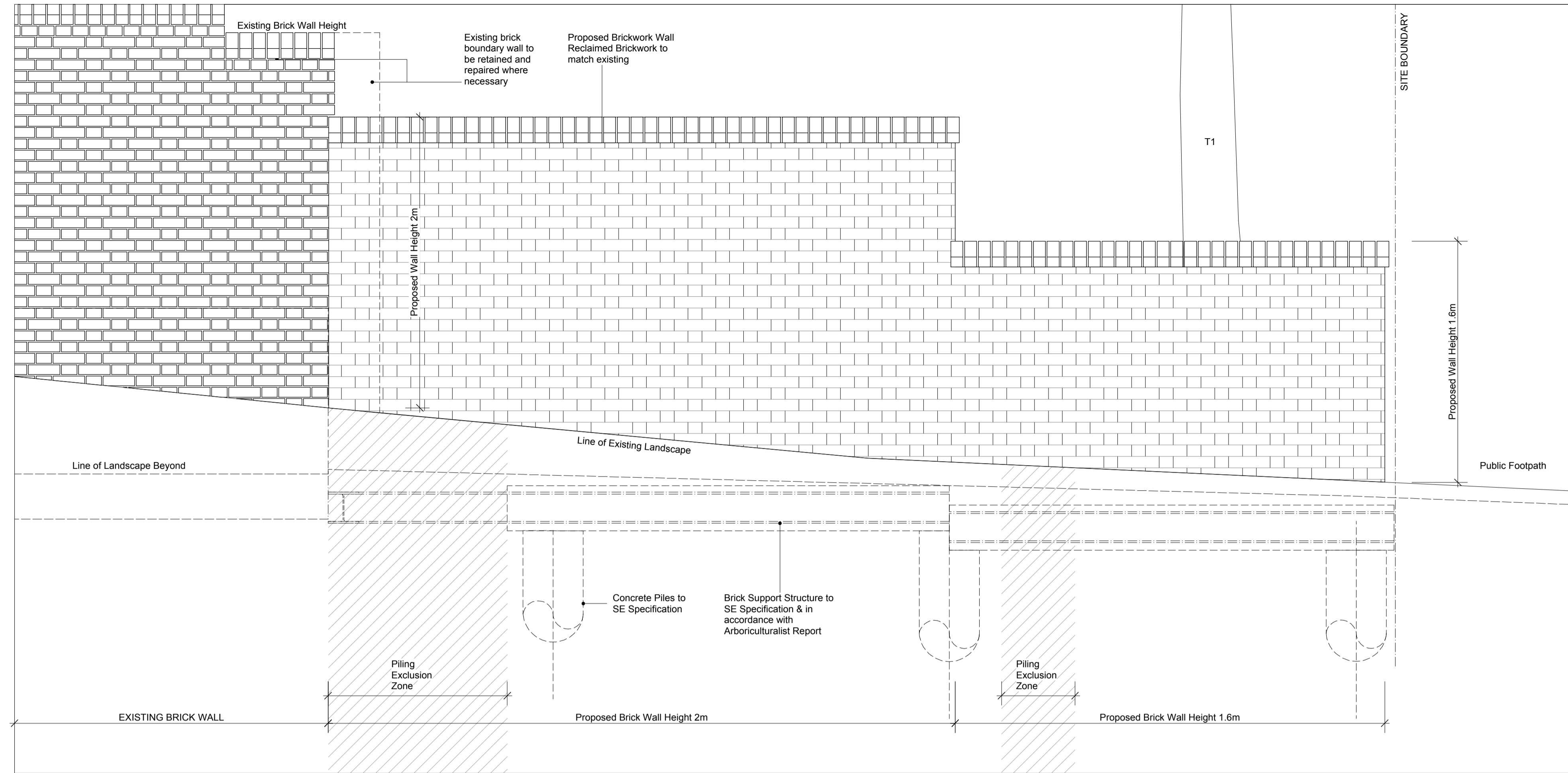
1 Proposed West Fence Elevation
