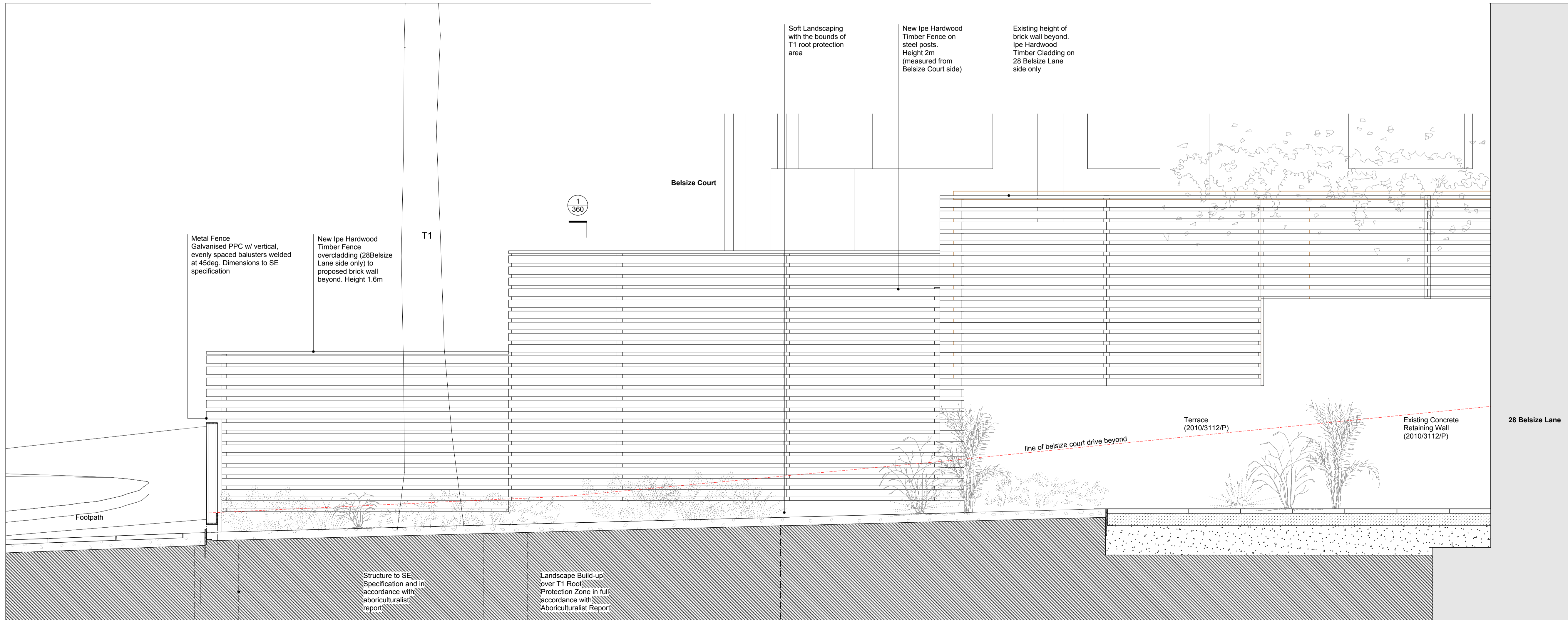
1 Proposed West Fence Elevation
