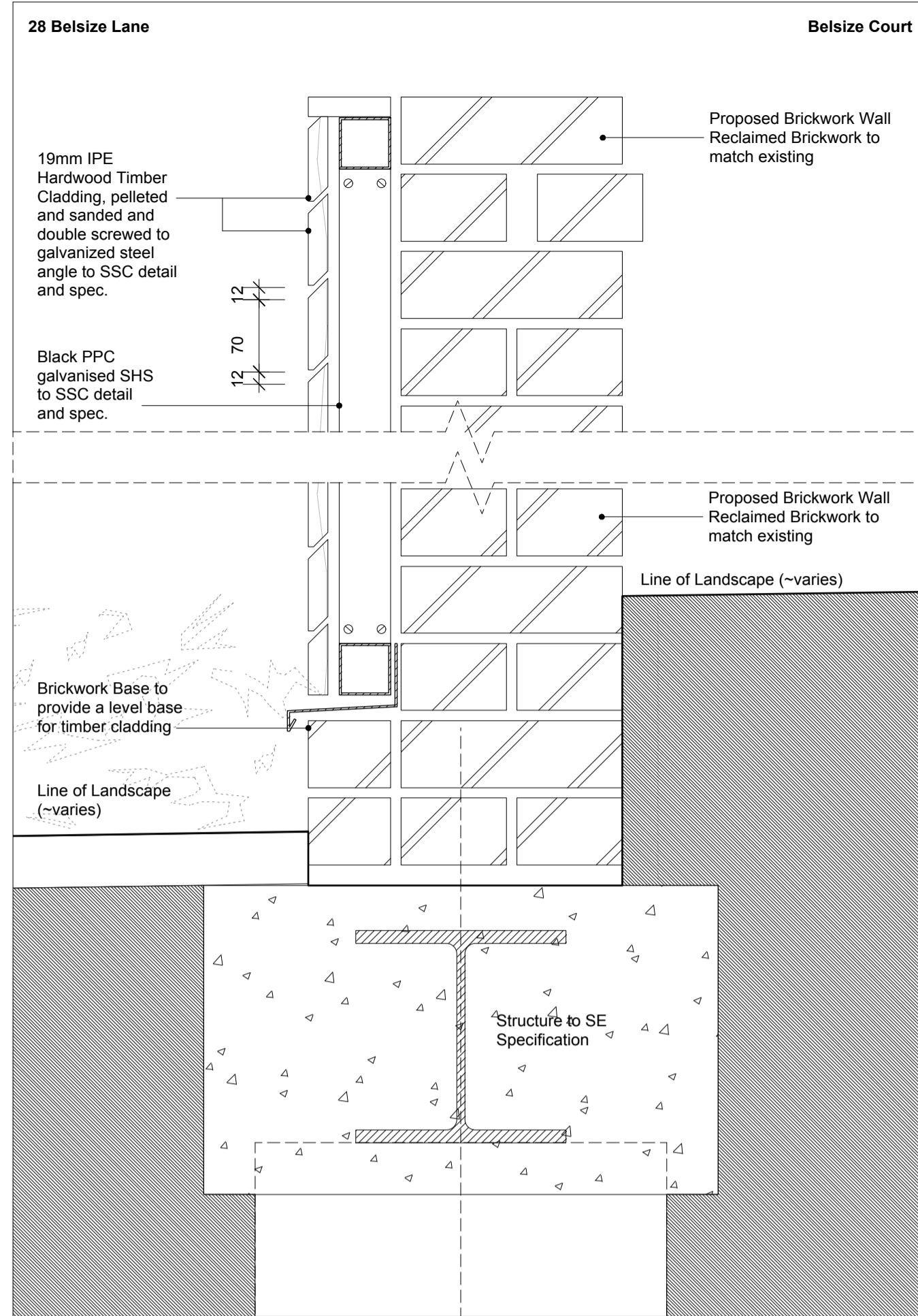
1 Proposed West Wall Detail
