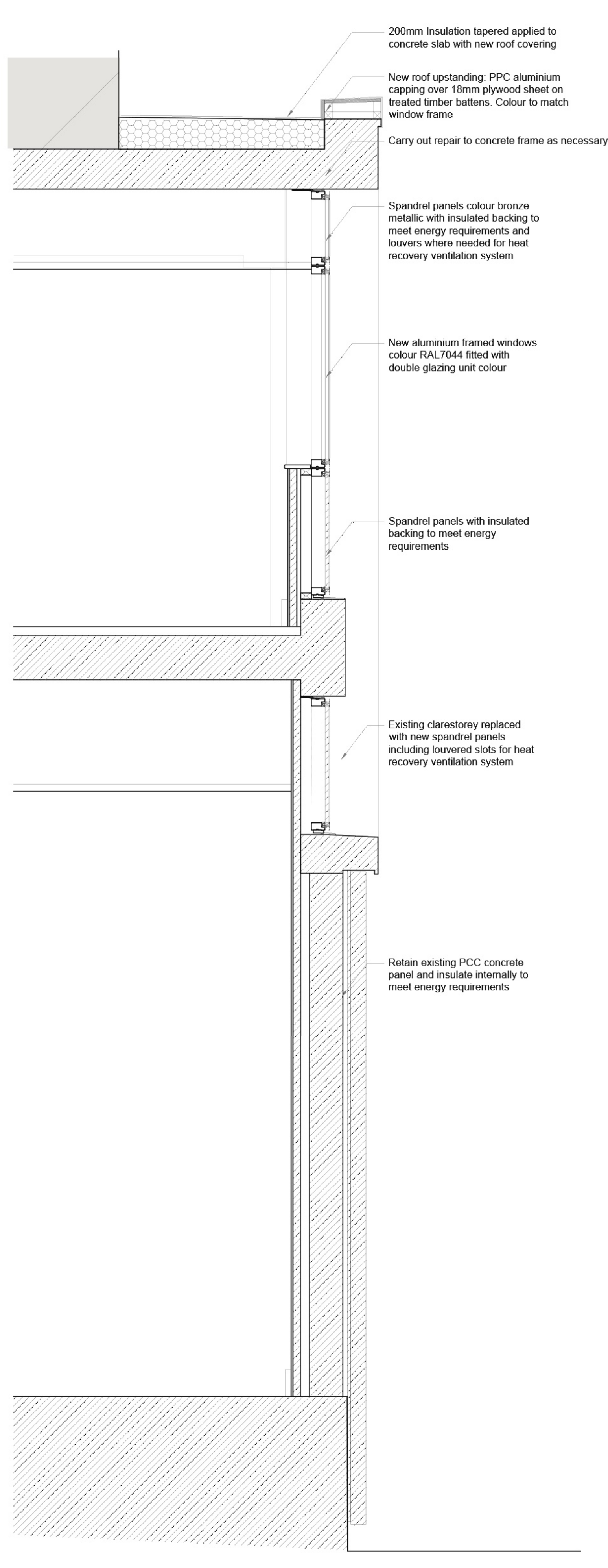
2 Section X-X SCALE 1:20 @ A1
