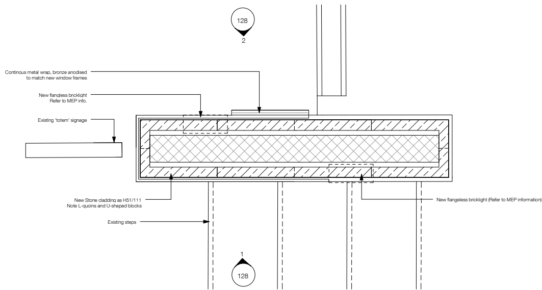
4 New Signage Monolith (G38) Plan 1 : 10
