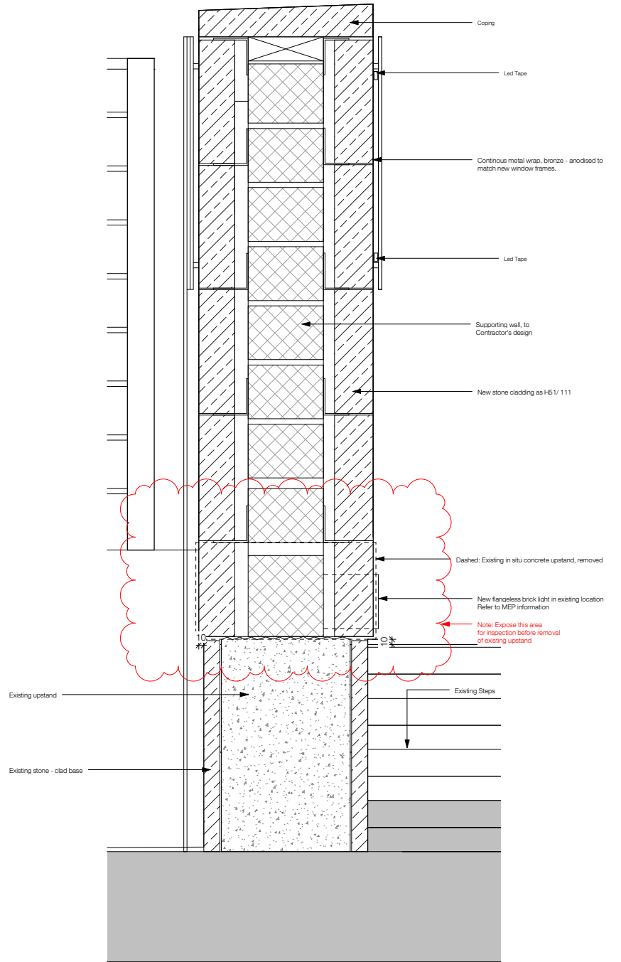
3 New Signage Monolith (G38) Section 1 : 5
