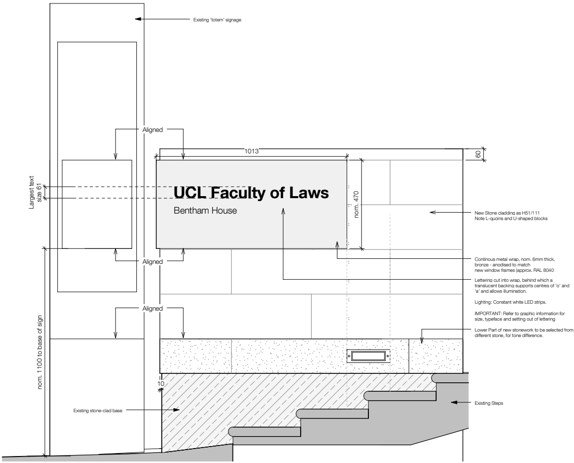
1 New Signage Monolith (G38) Elevation 1 1 : 10
