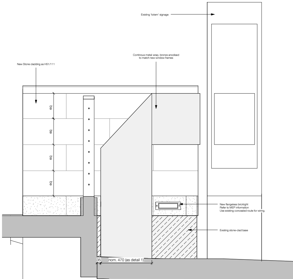
2 New Signage Monolith (G38) Elevation 2 1 : 10
