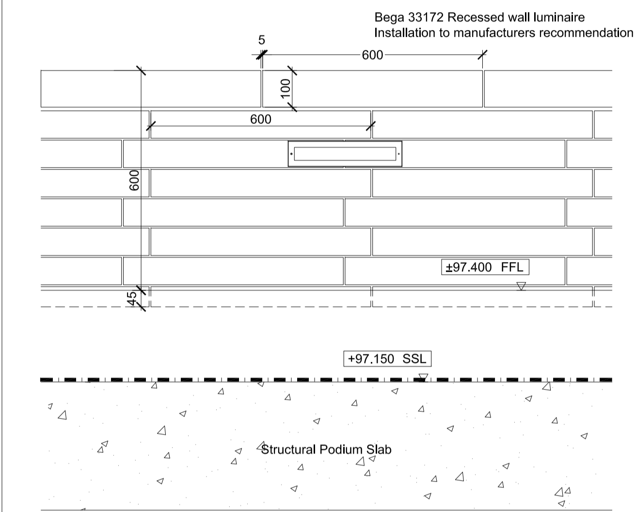
3 Wall Recessed Light - Elevation Scale 1:10
