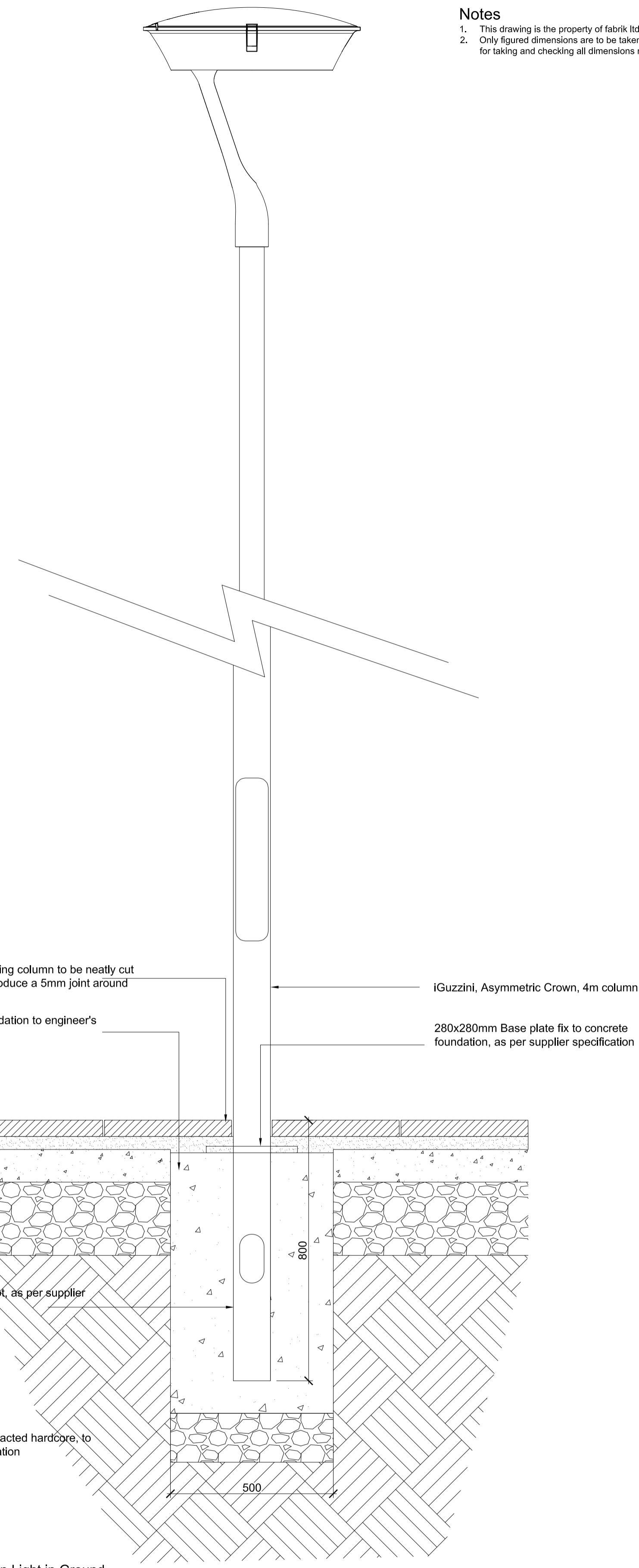
7 Column Light in Ground Scale 1:10
