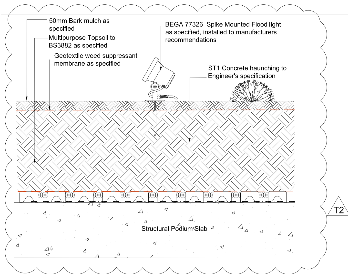
1 Tree uplighter Scale 1:10
