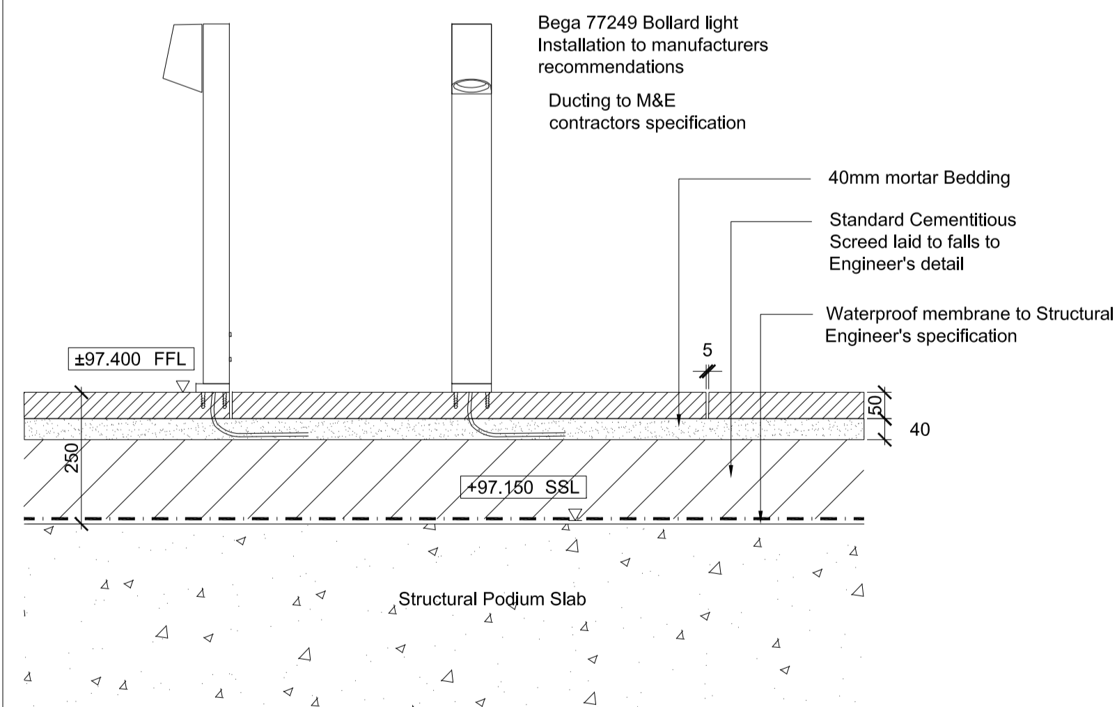
5 Bollard Light over Podium Scale 1:10
