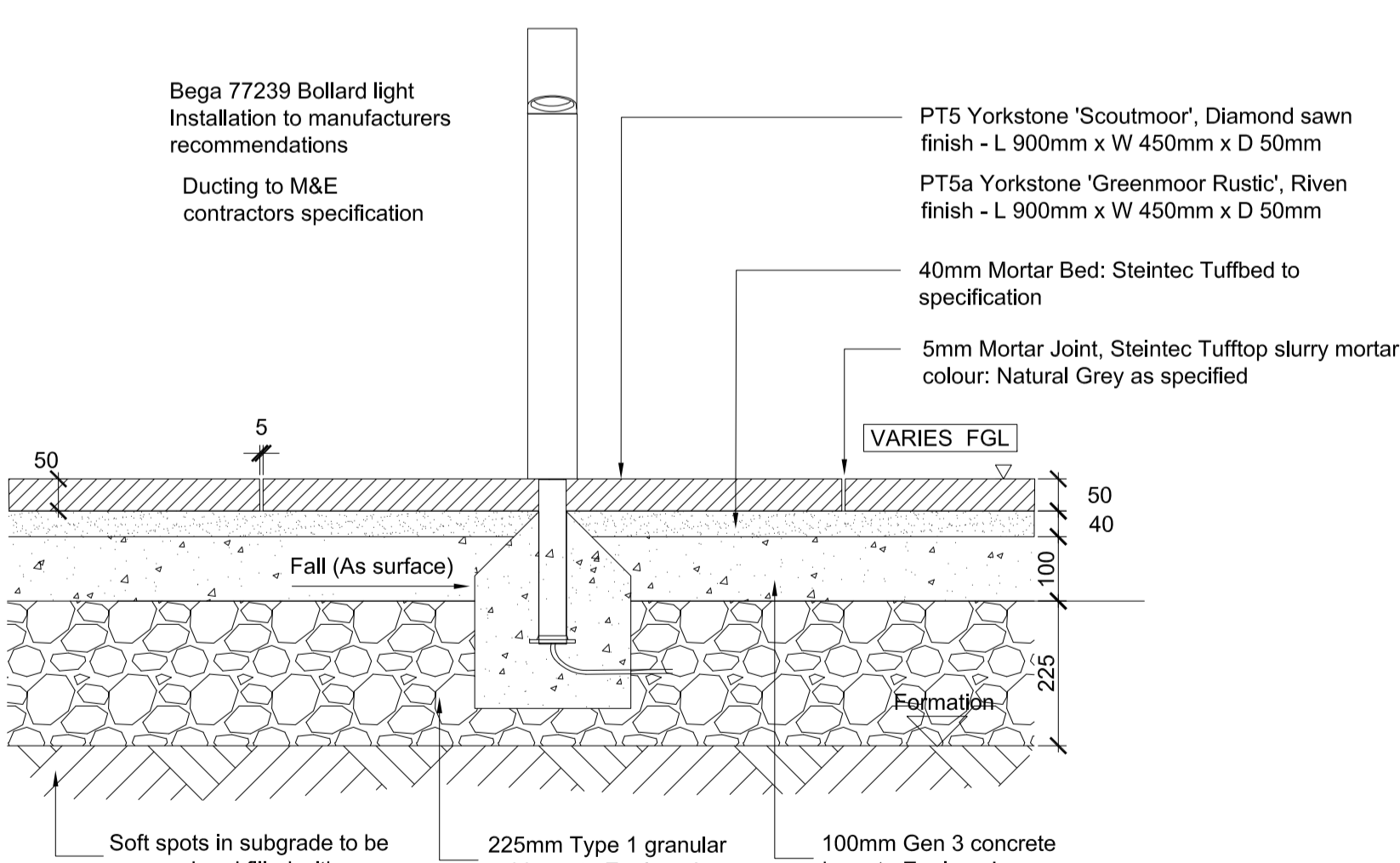
6 Bollard Light in Ground Scale 1:10
