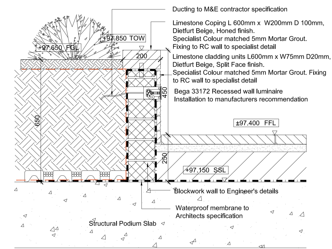
4 Wall Recessed light - Section Scale 1:10
