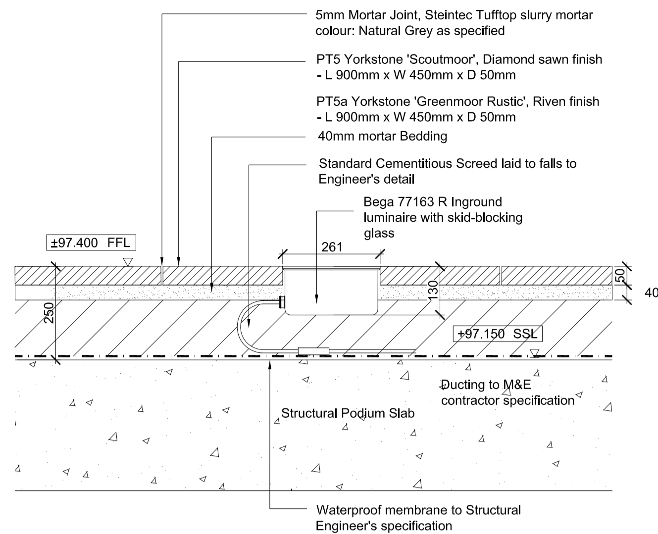
2 Inground uplighter in paving Scale 1:10
