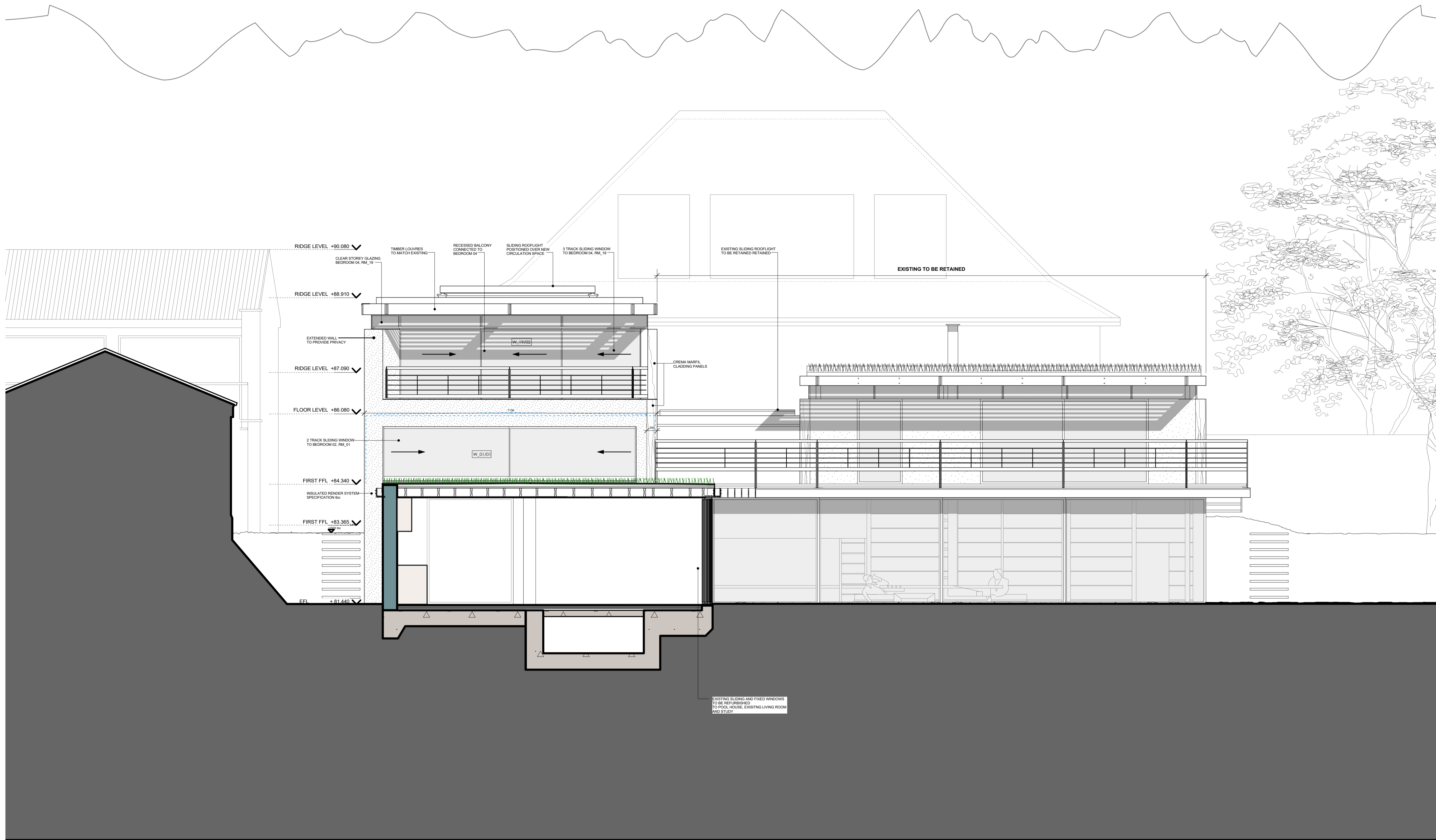
01 PROPOSED SOUTH WEST ELEVATION / SECTION 210 SCALE: 1:50 @ A1
