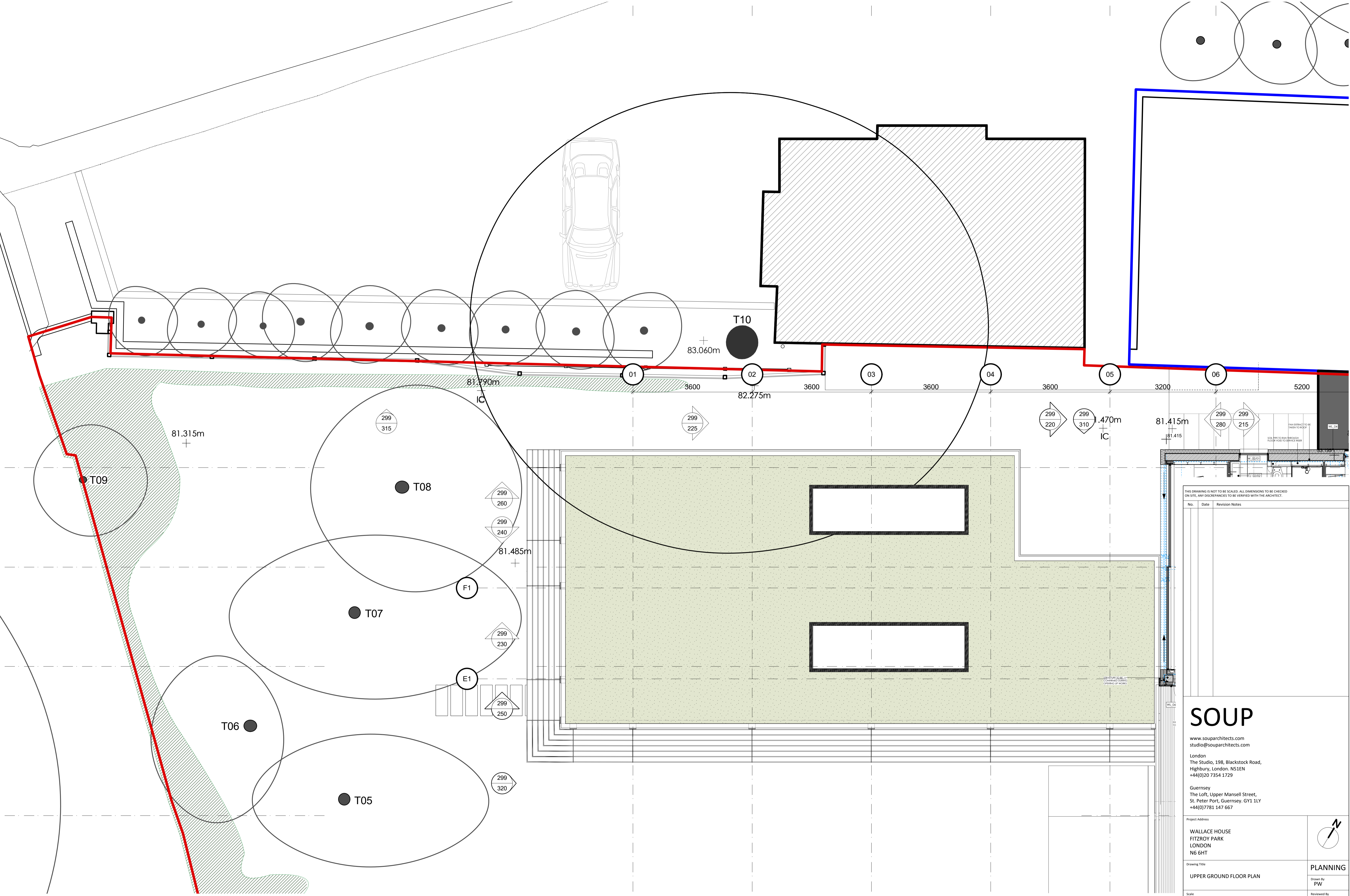
01 PROPOSED GROUND FLOOR PLAN SCALE: 1:50 @ A1
