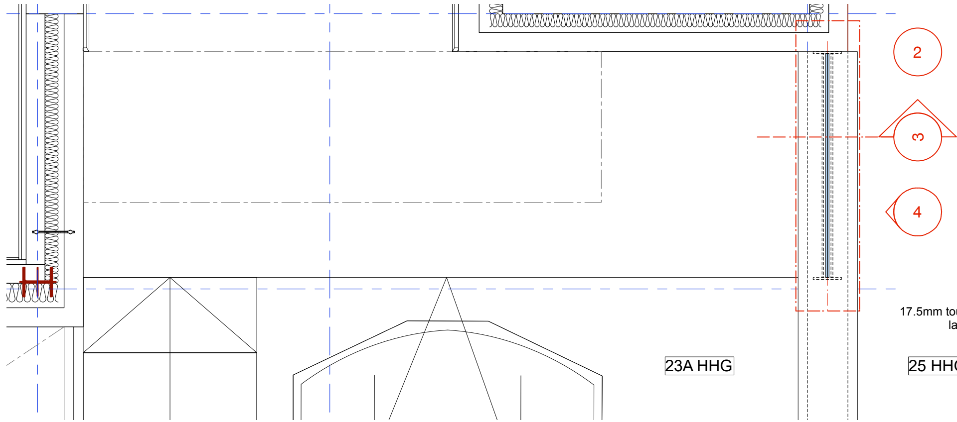
1 GF drive_plan Scale: 1:20
