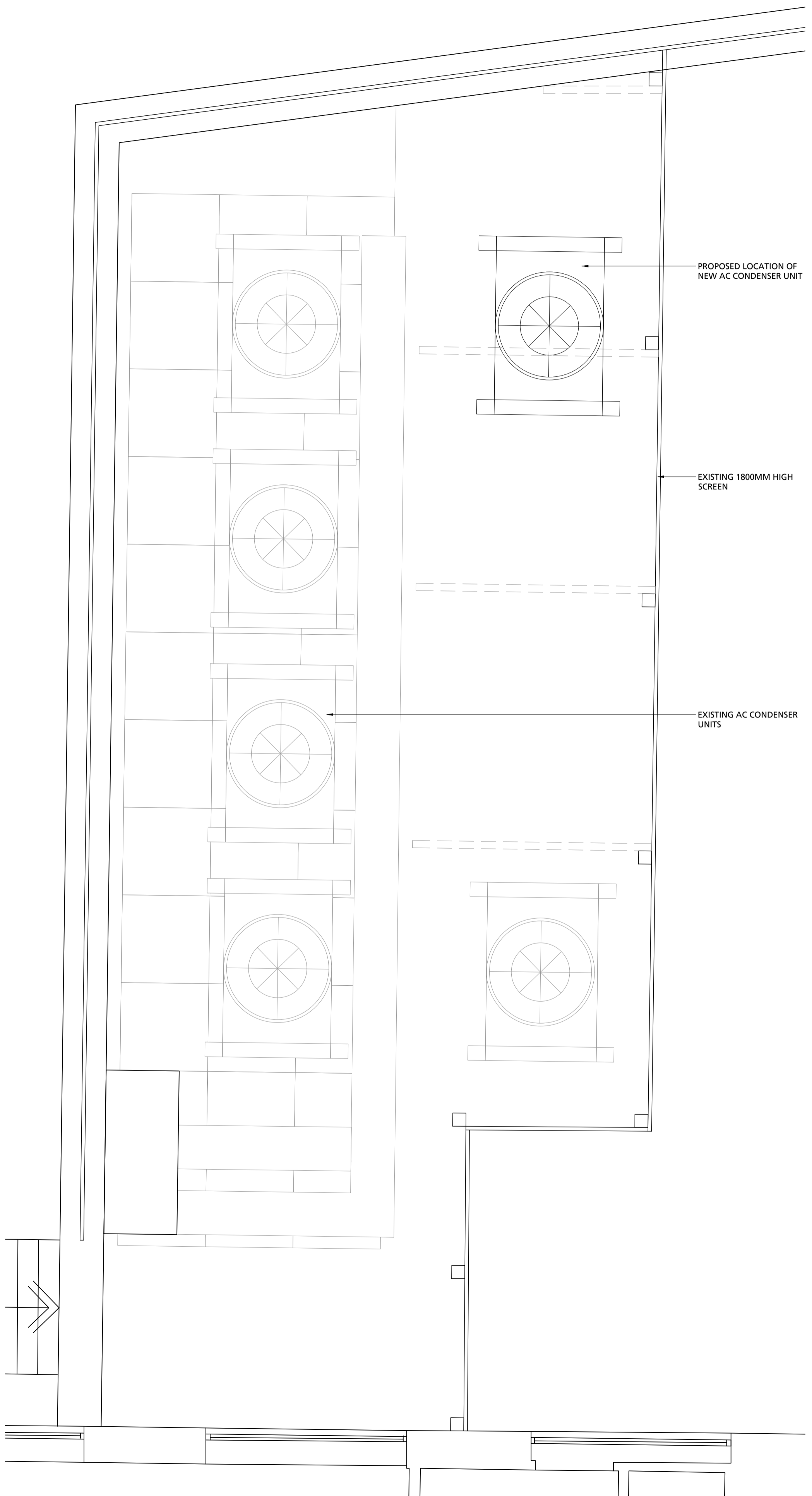
GA FOURTH FLOOR ROOF PLAN - PLAN SCALE 1:20
