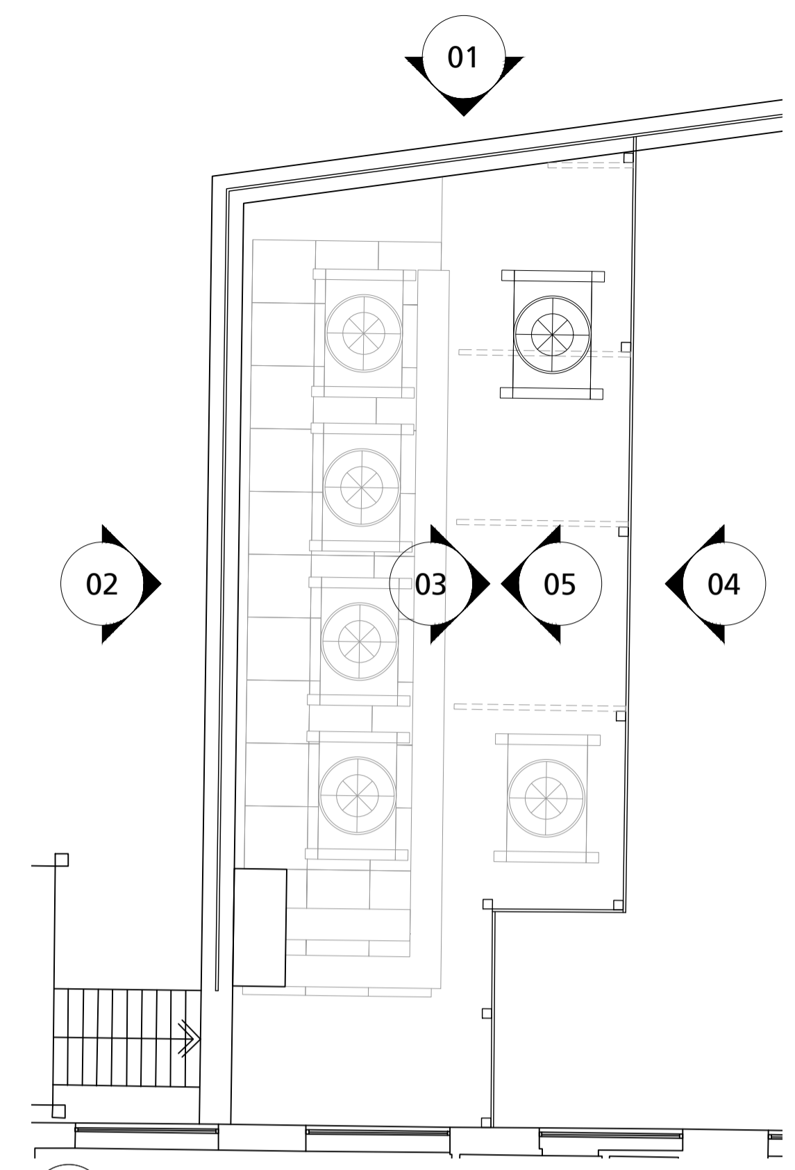
RP FOURTH FLOOR ROOF PLAN - KEY PLAN SCALE 1:50
