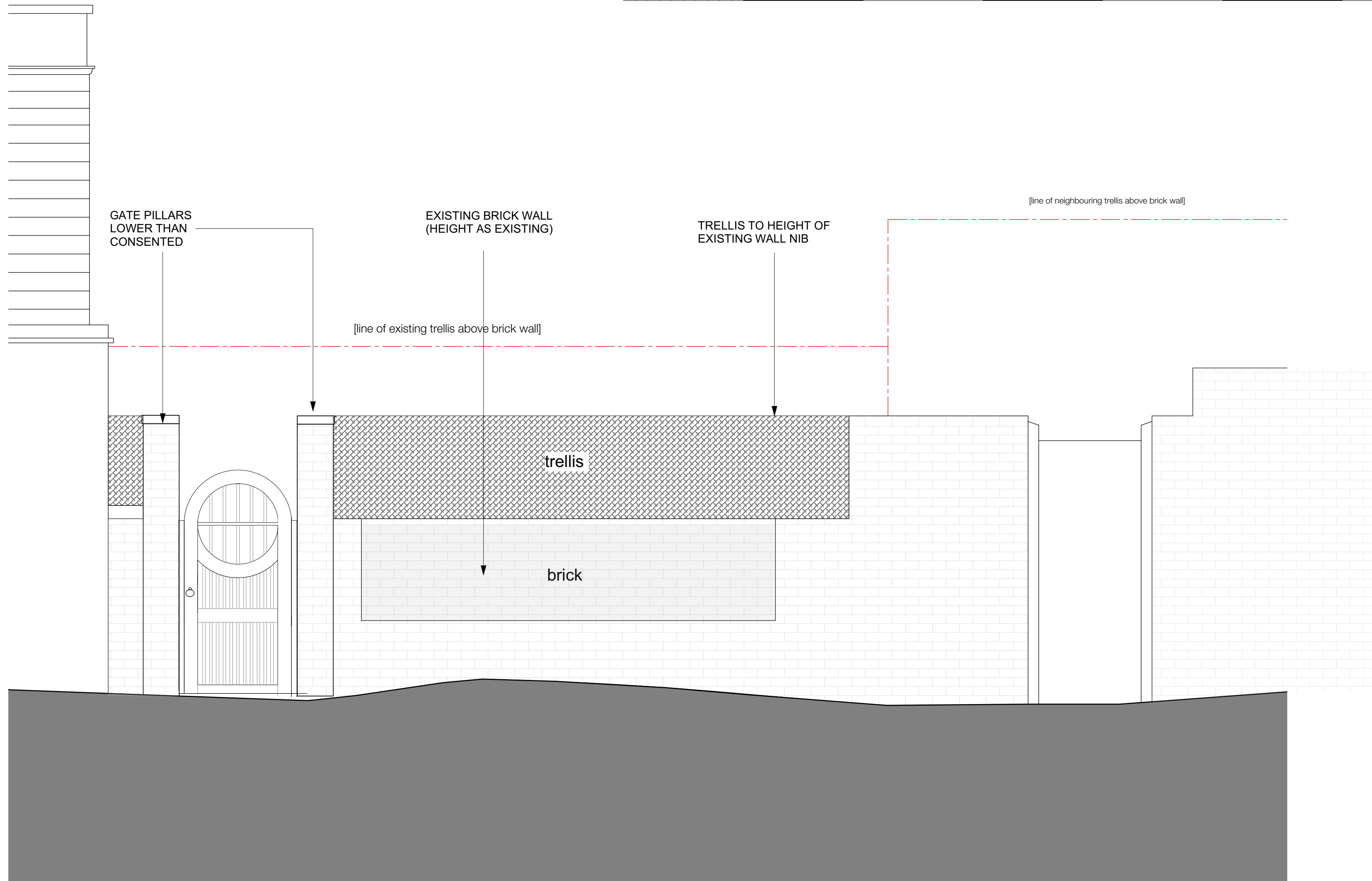
Proposed rear wall elevation
