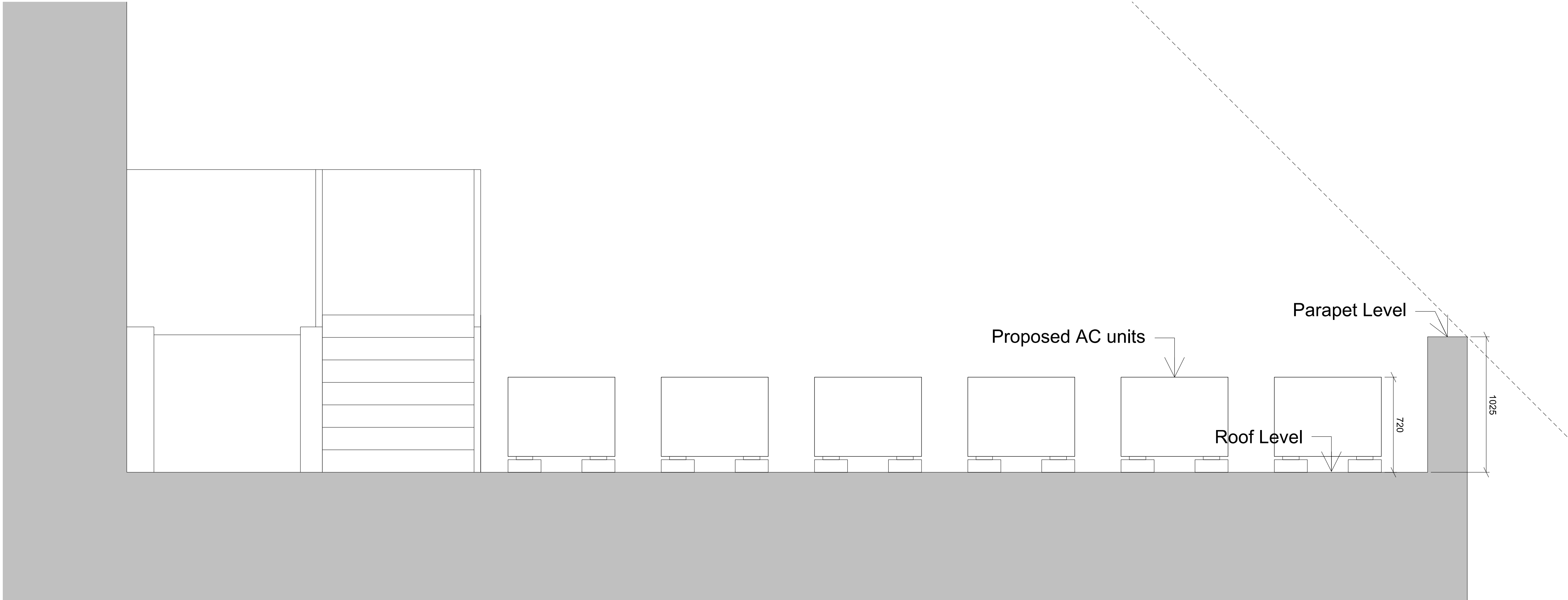
SECTION 01 - PROPOSED
