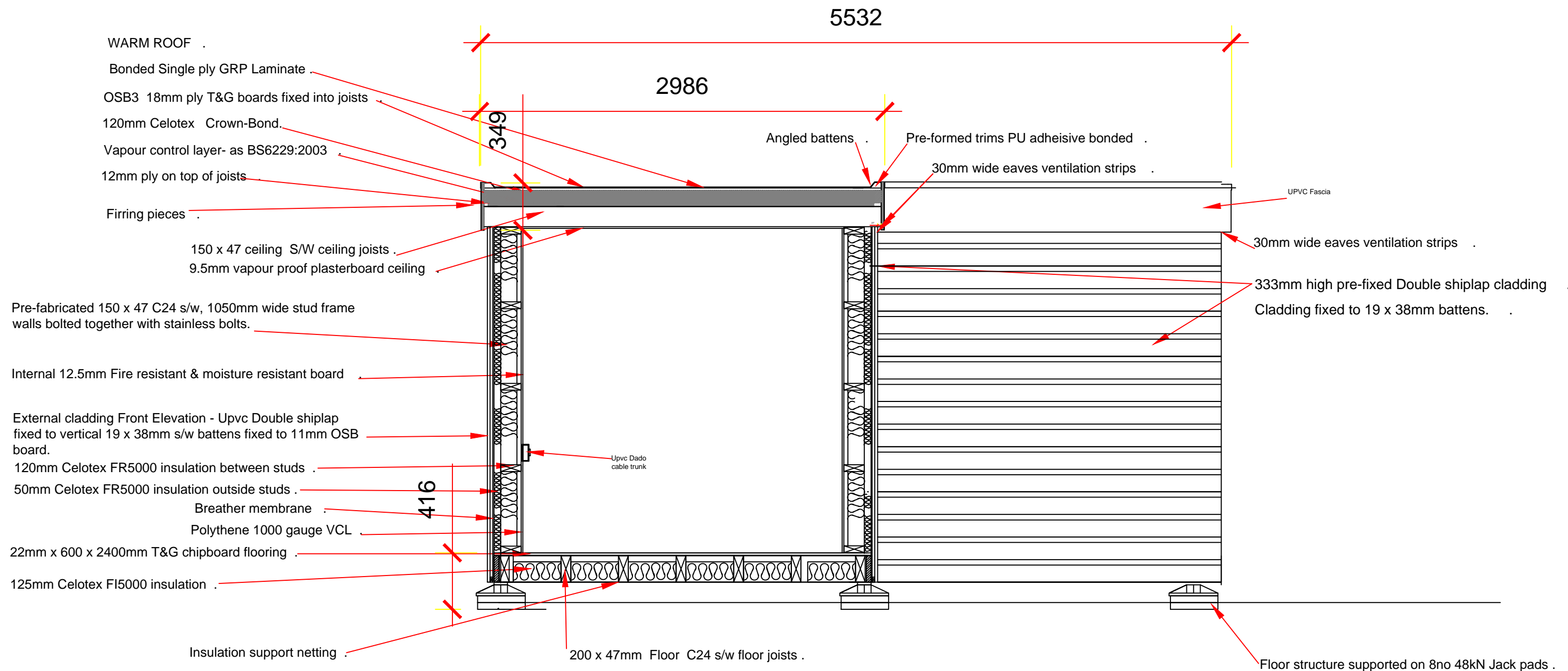
Front Section A - A
