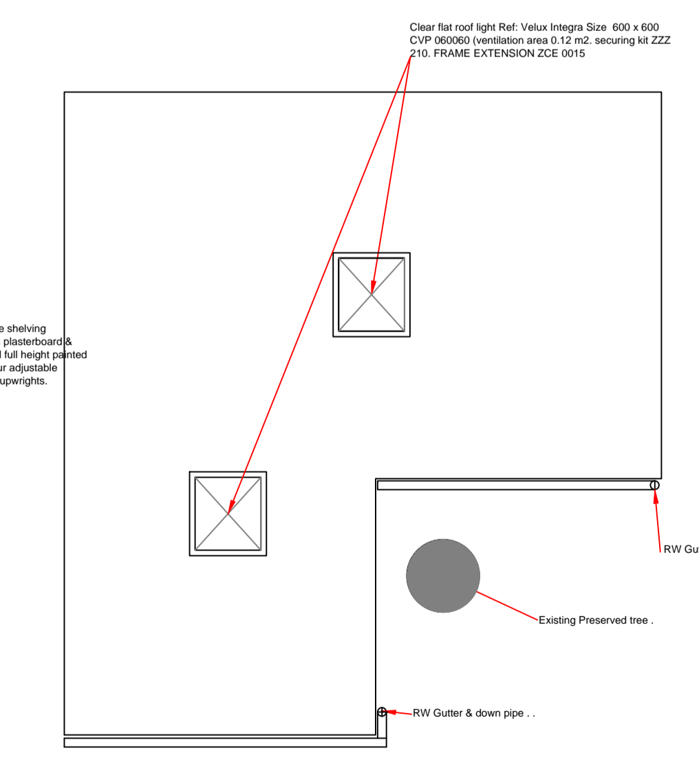
ROOF PLAN LAYOUT
