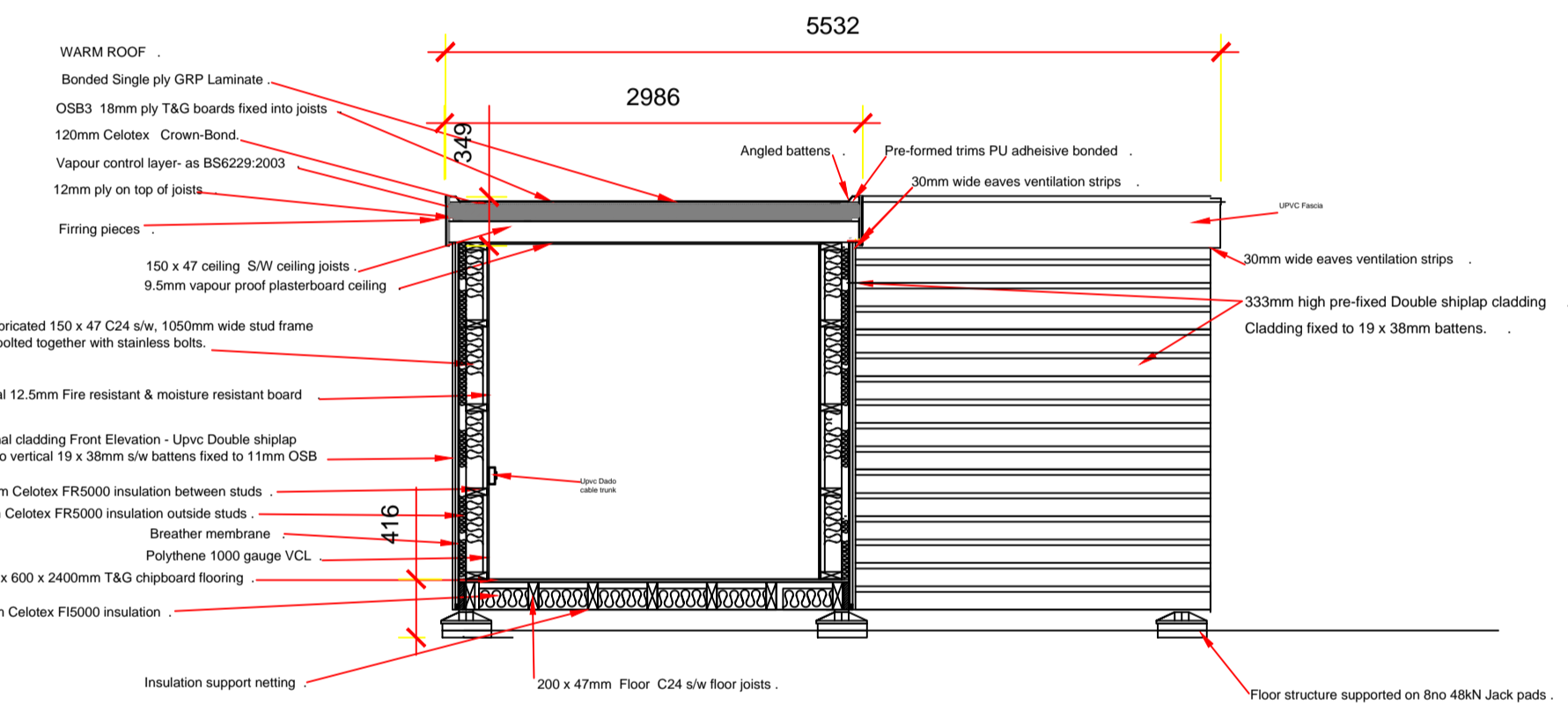
Front Section A - A
