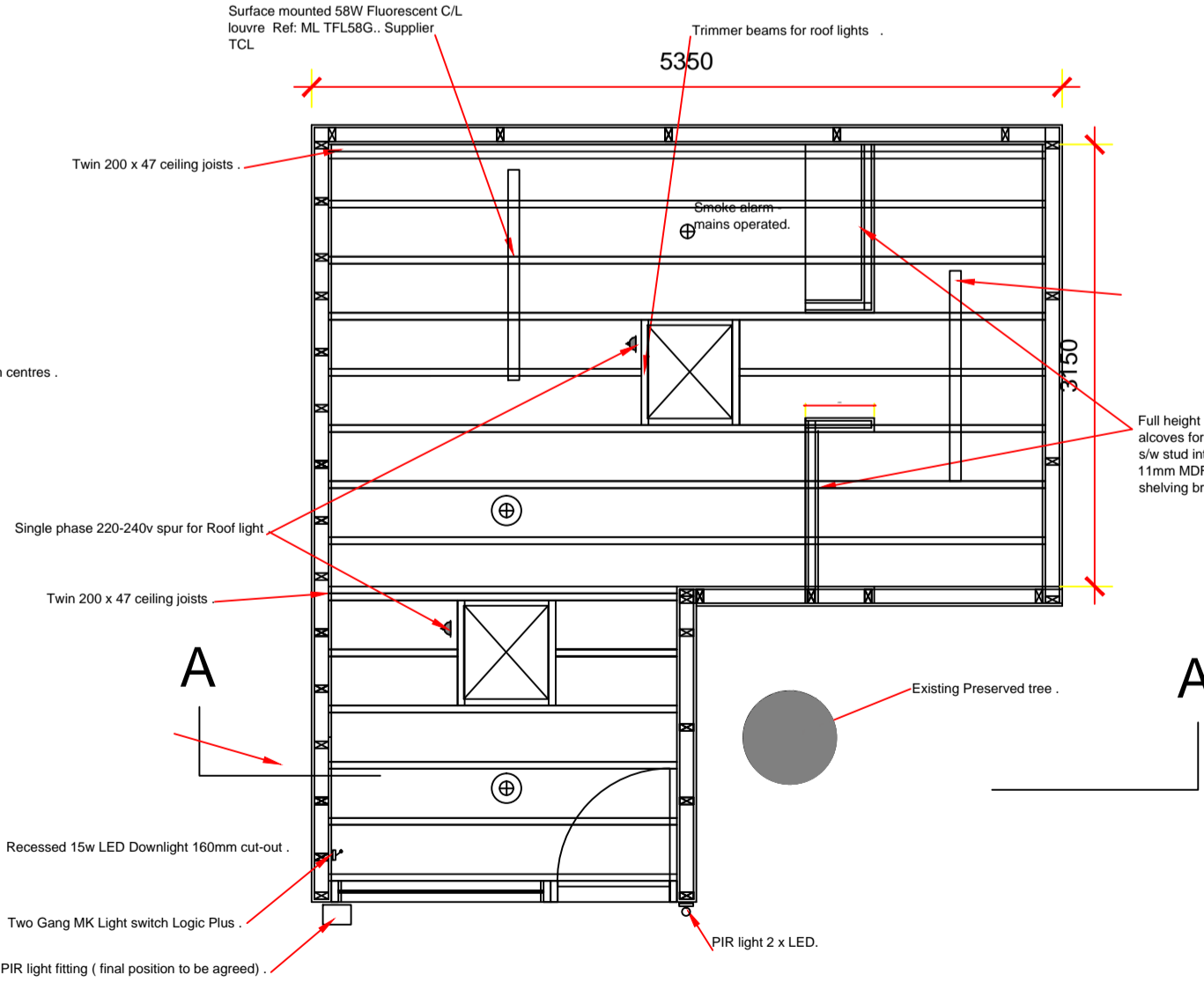
CEILING & LIGHTING LAYOUT
