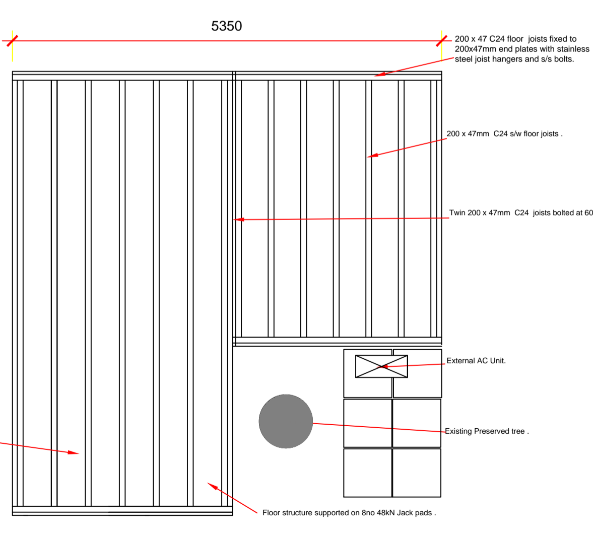
FLOOR JOIST LAYOUT
