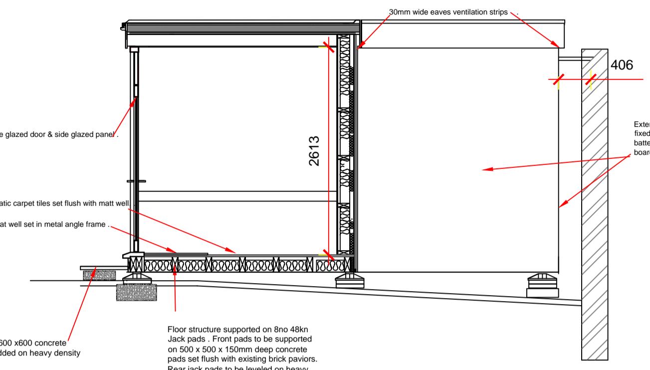
SIDE SECTION B - B
