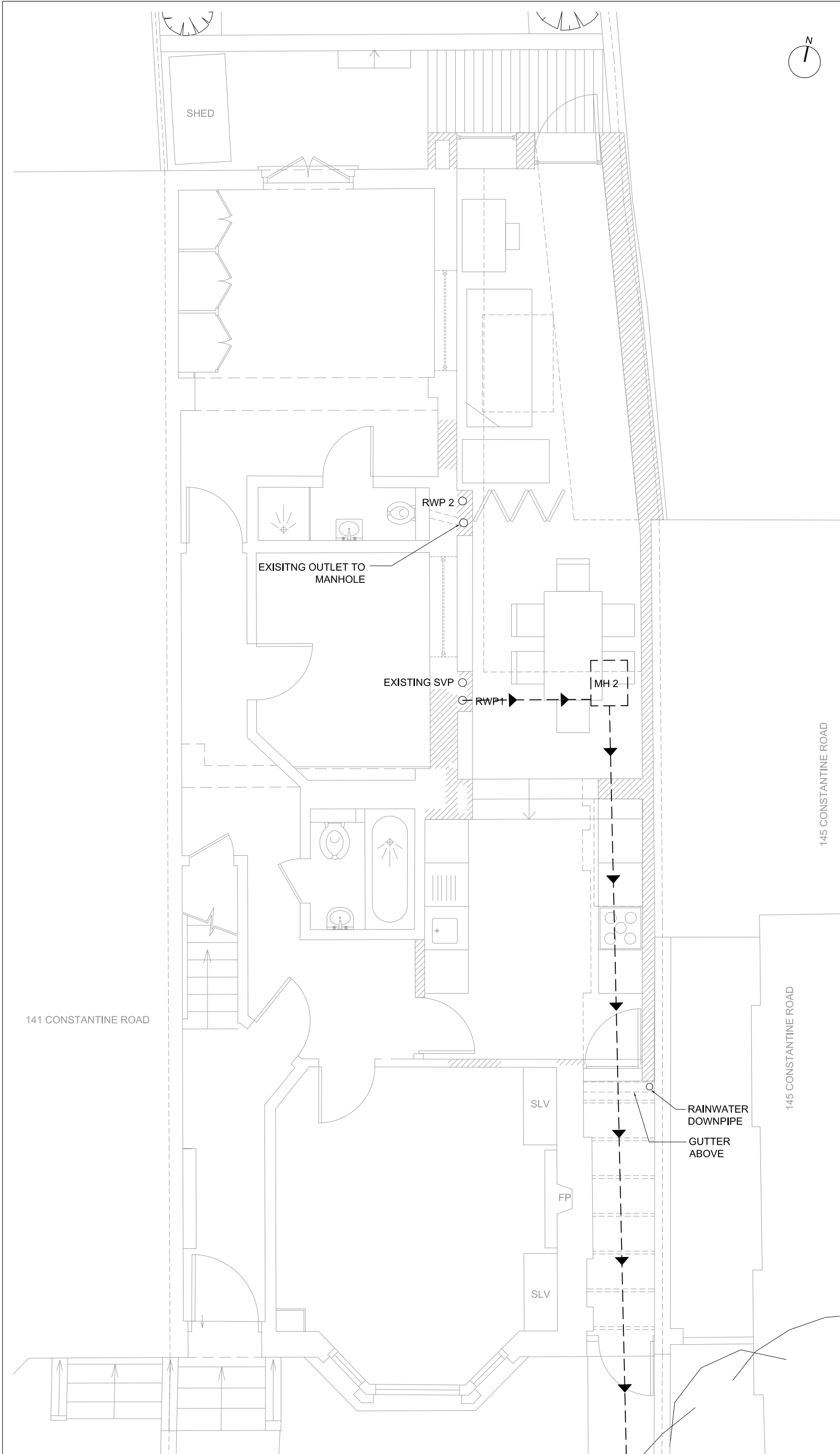
PROPOSED DRAINAGE GROUND FLOOR PLAN
