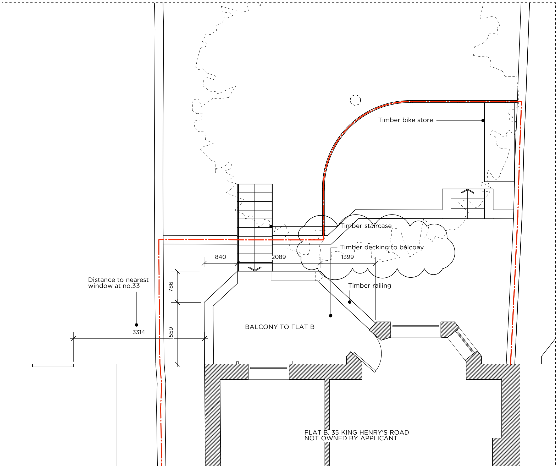
1. PROPOSED BALCONY PLAN
