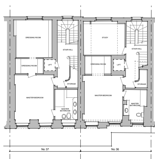
8 SECOND FLOOR PLAN YEAR : 2009 PL-33
