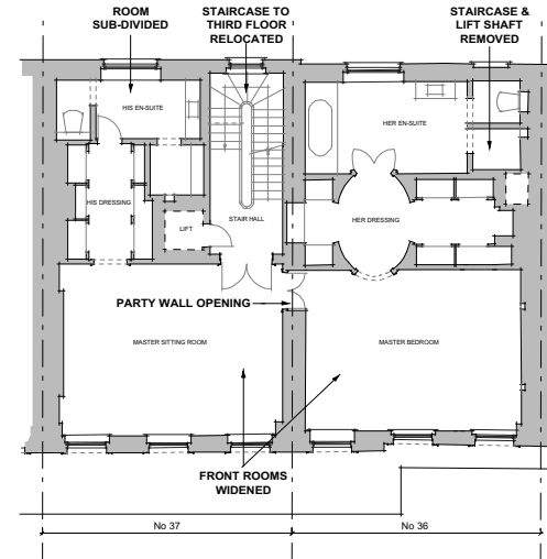
9 SECOND FLOOR PLAN YEAR : 2017 (EXISTING) PL-33
