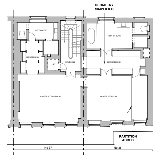
10 SECOND FLOOR PLAN PROPOSED PL-33
