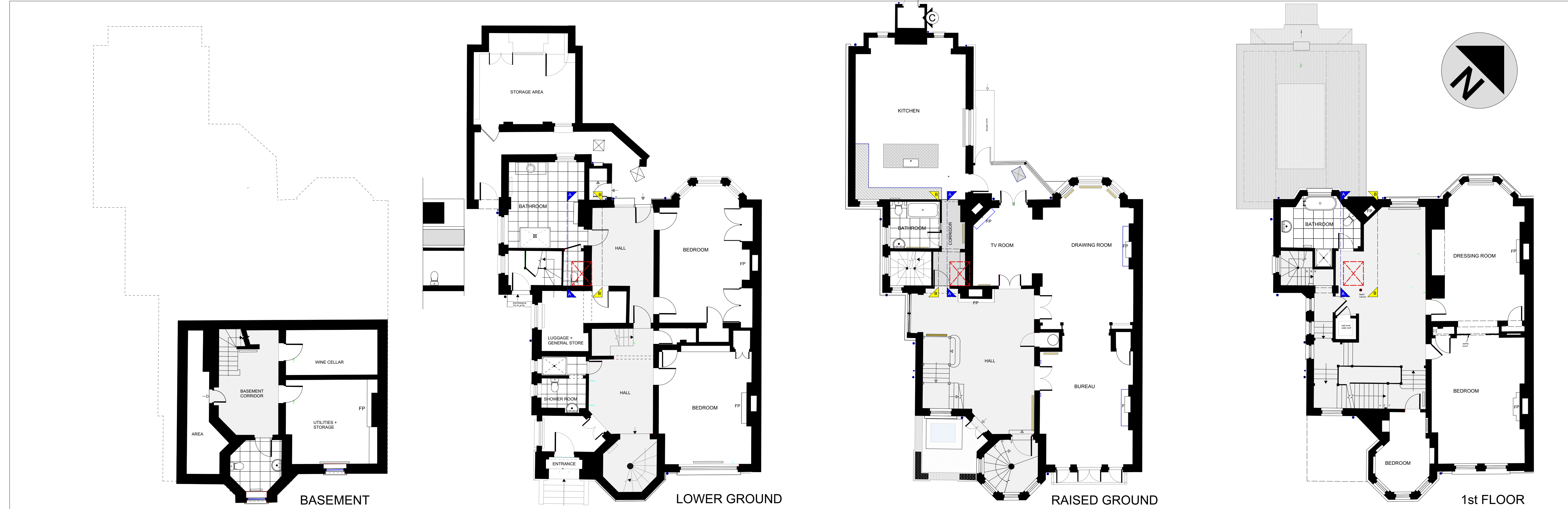
EXISTING PLANS
