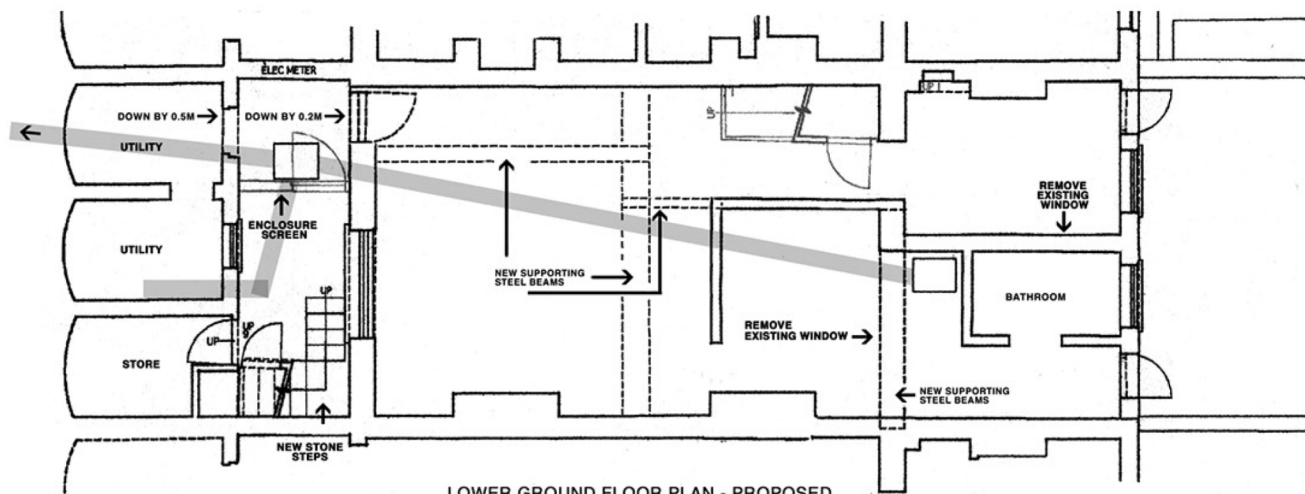
LOWER GROUND FLOOR PLAN - PROPOSED
