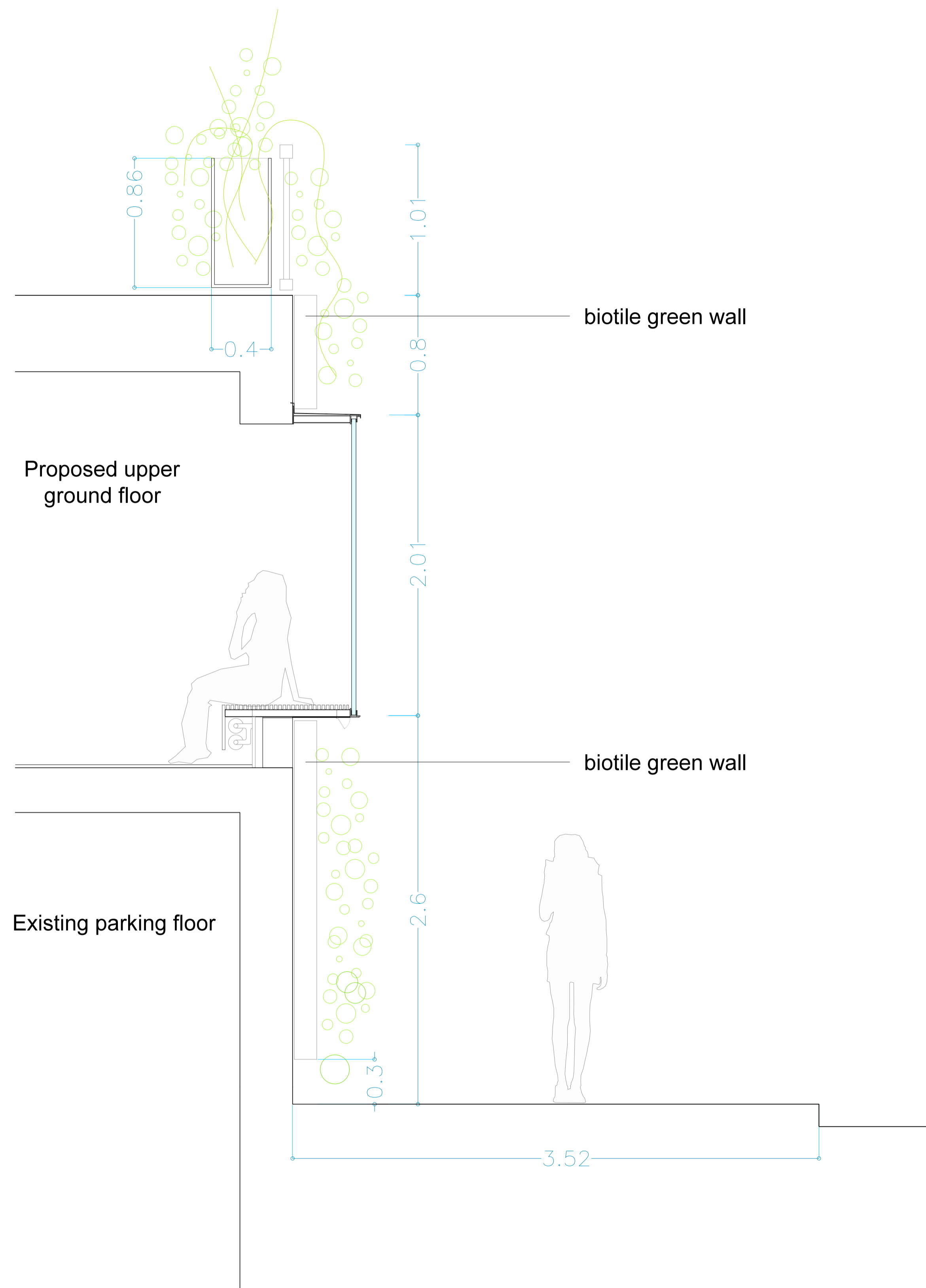
PROPOSED DETAILED SECTION CC sc 1:20
