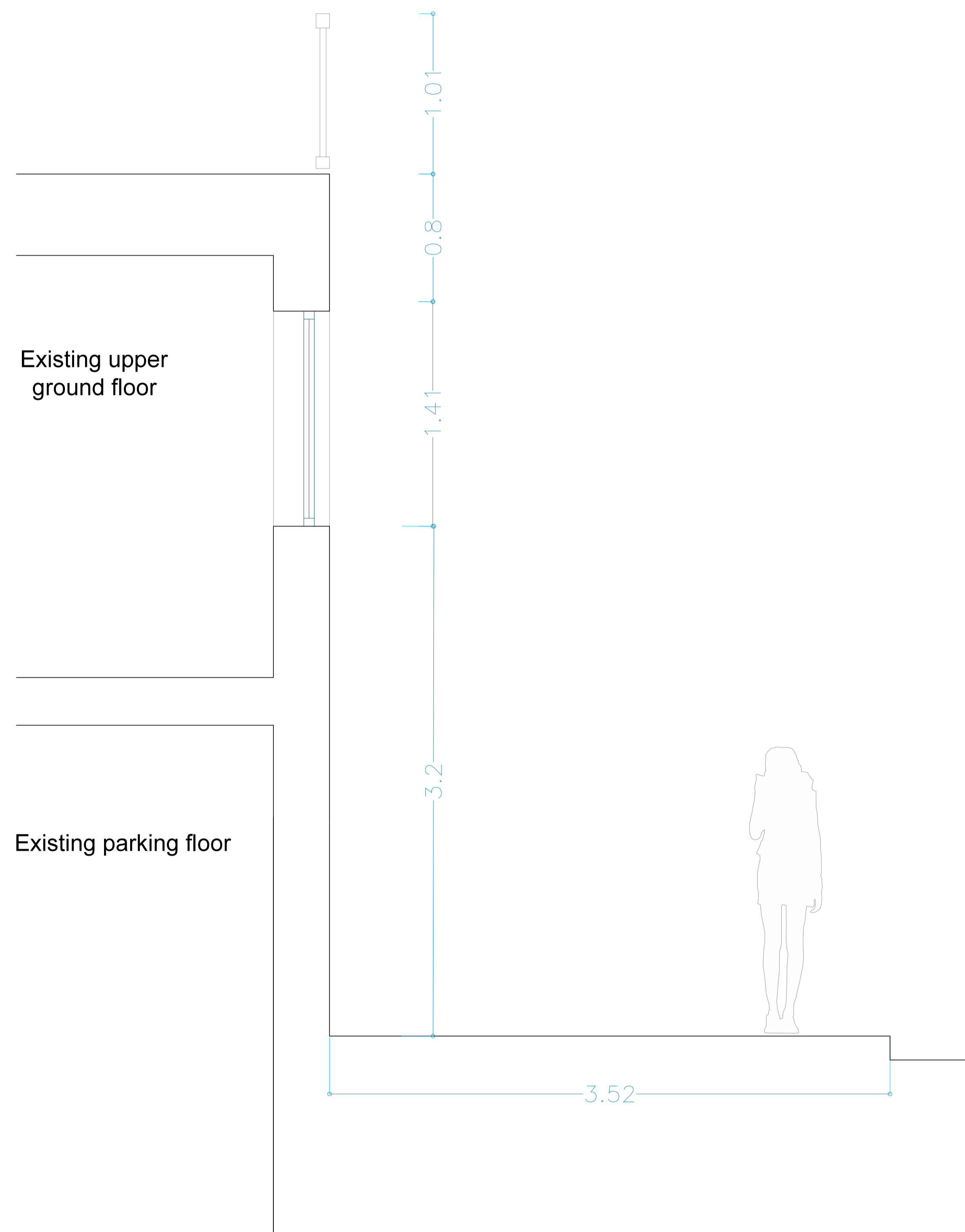
EXISTING DETAILED SECTION CC sc 1:20
