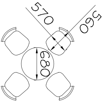
Dimension of Chair & Table
