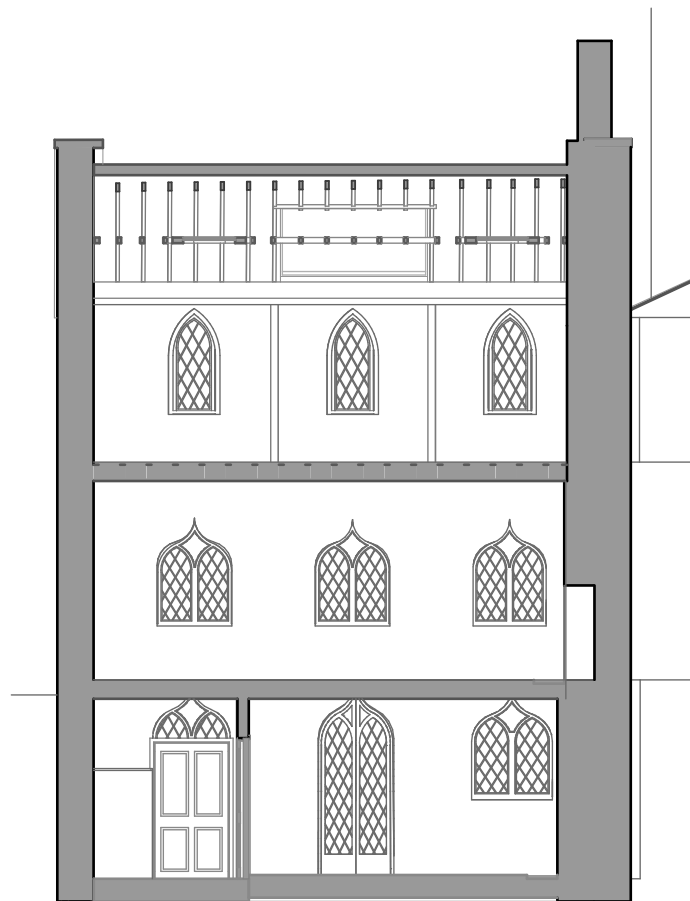
S-08 Building Section 1:100
