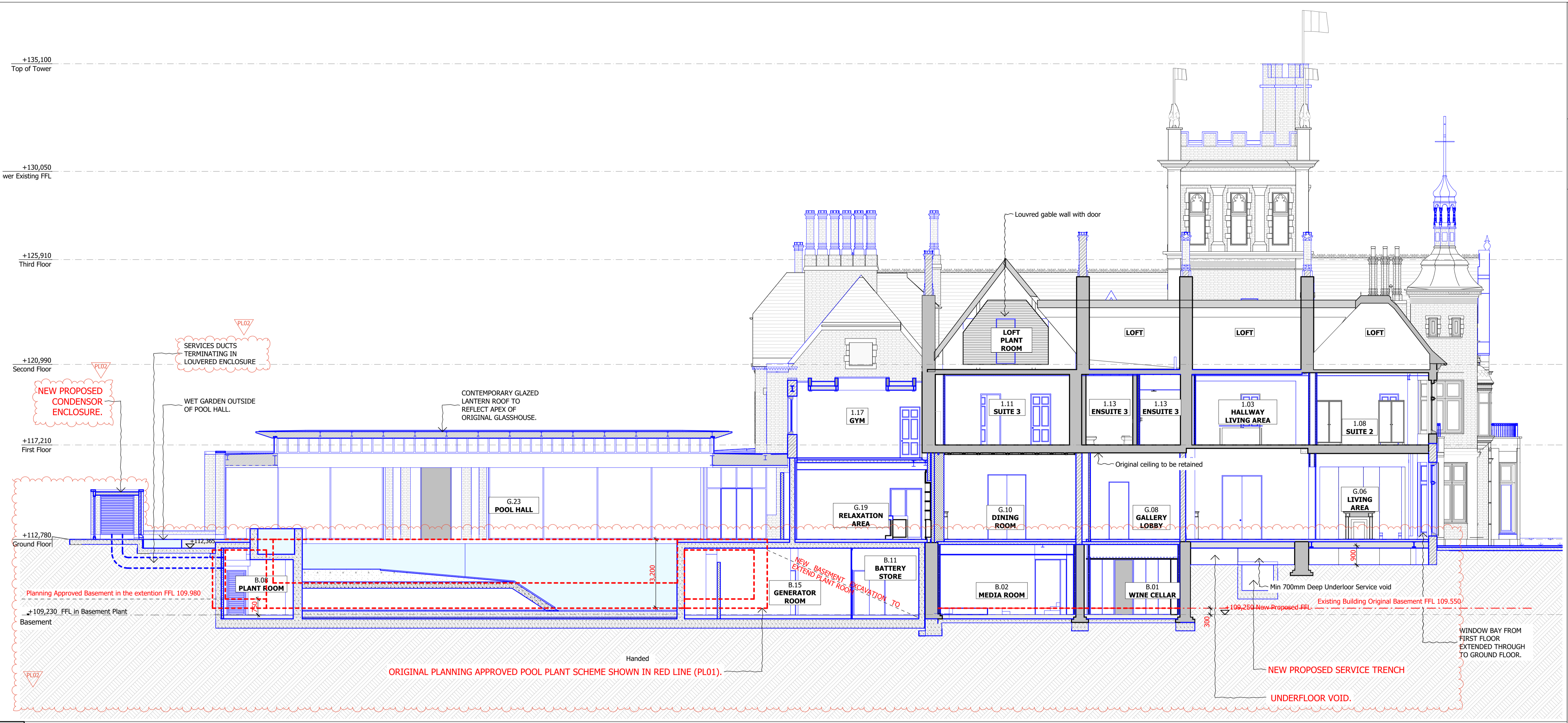
1 LONG SECTION DD - PROPOSED
