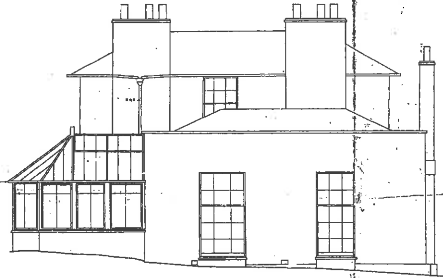
EAST ELEVATION
