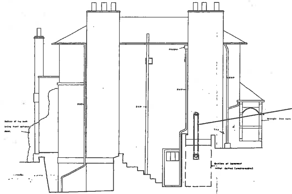
WEST ELEVATION
