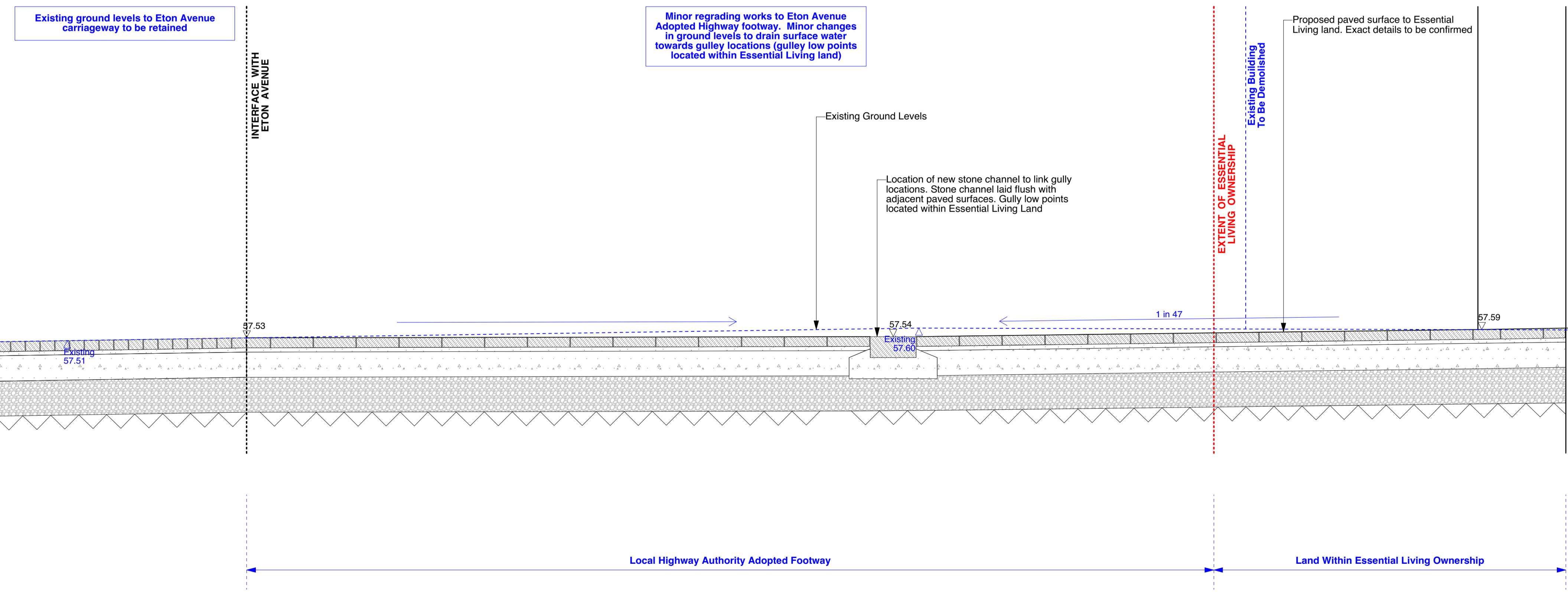
Section Through Proposed Interface With Eton Avenue Footway Scale: 1:20 at A1
