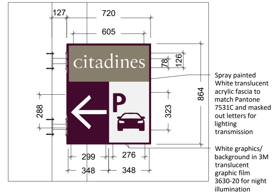
DETAIL A - GRAPHIC
