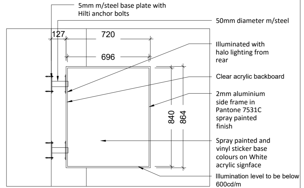
DETAIL A - FRONT SECTION
