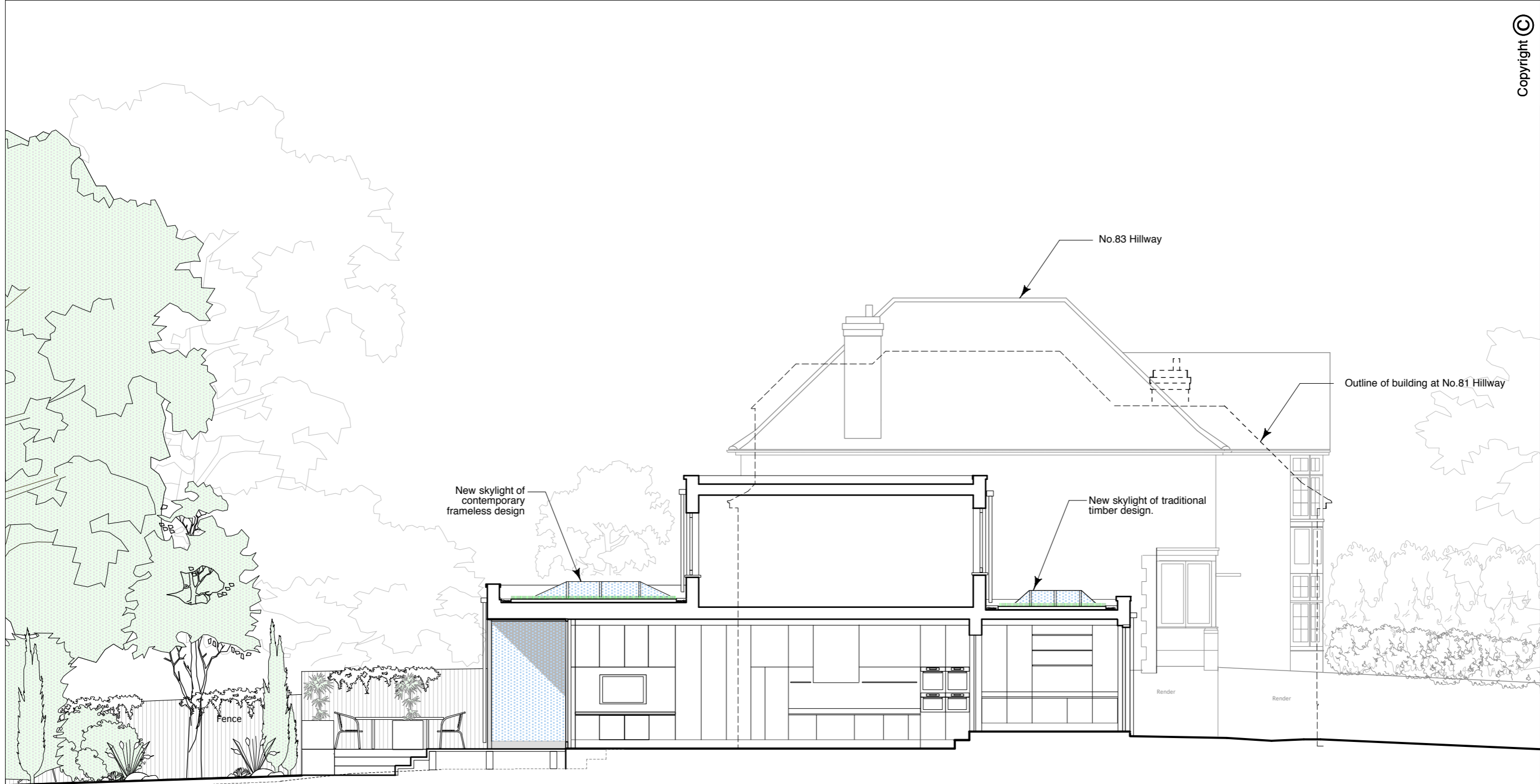
SECTION D-D - PROPOSED
