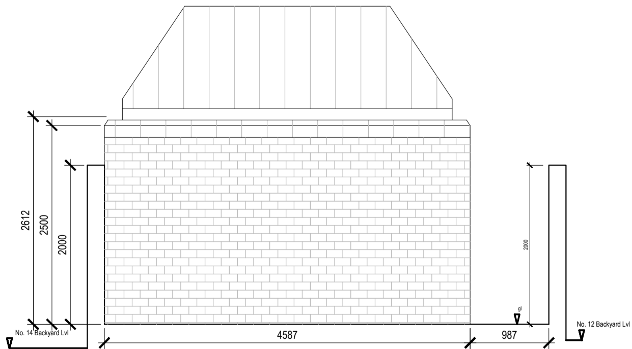
REAR ELEVATION
