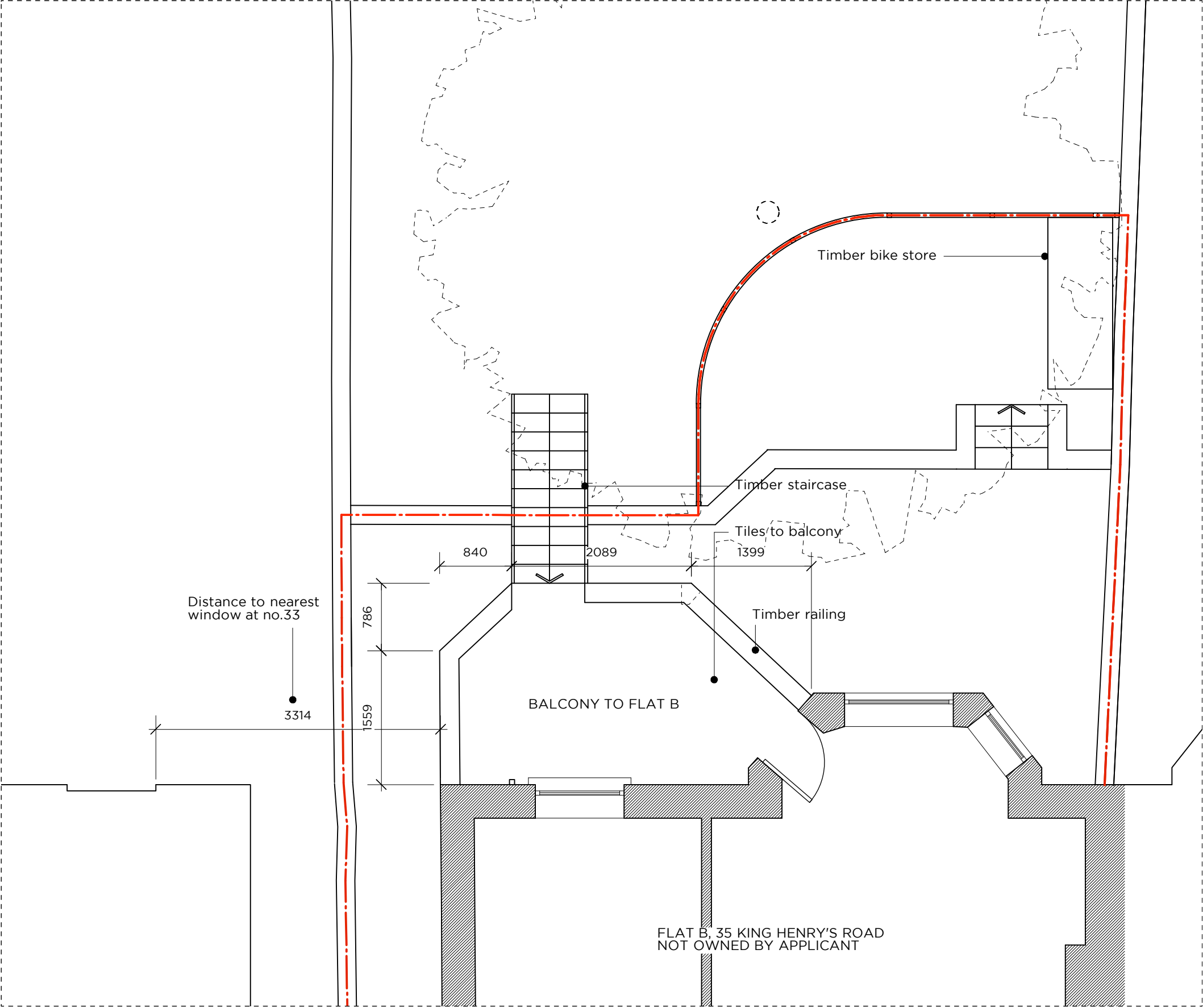
1. PROPOSED BALCONY PLAN
