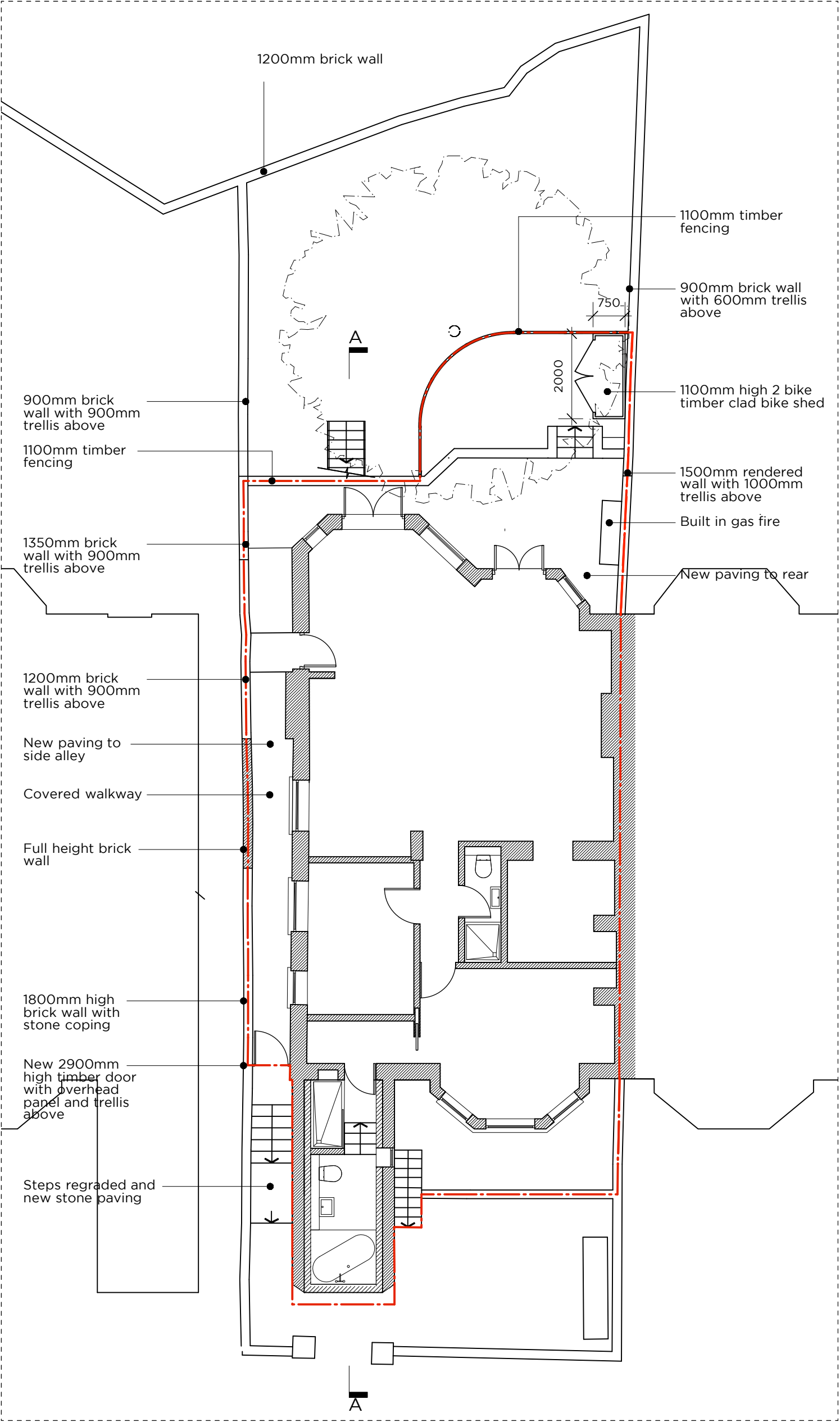
1. PROPOSED SITE PLAN
