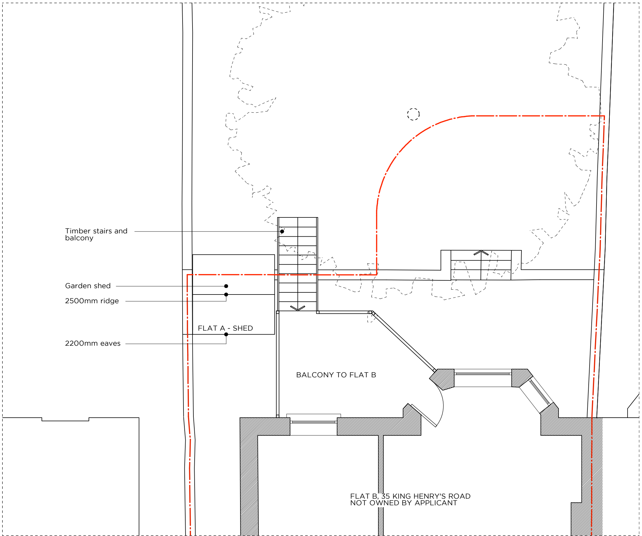
1. EXISTING BALCONY PLAN
