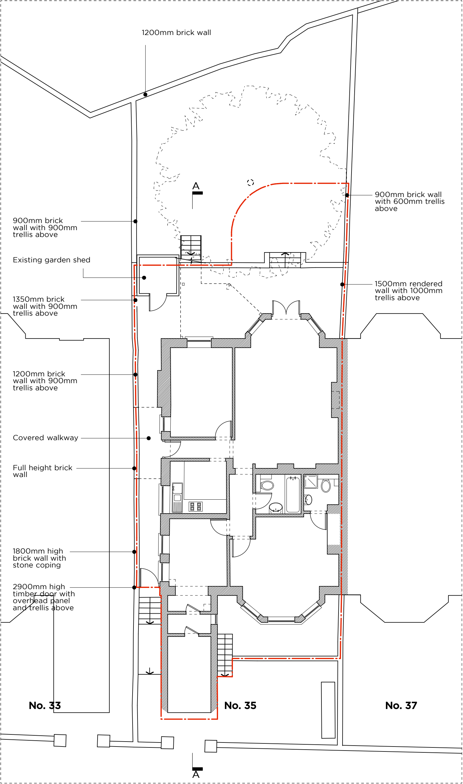
1. EXISTING SITE PLAN
