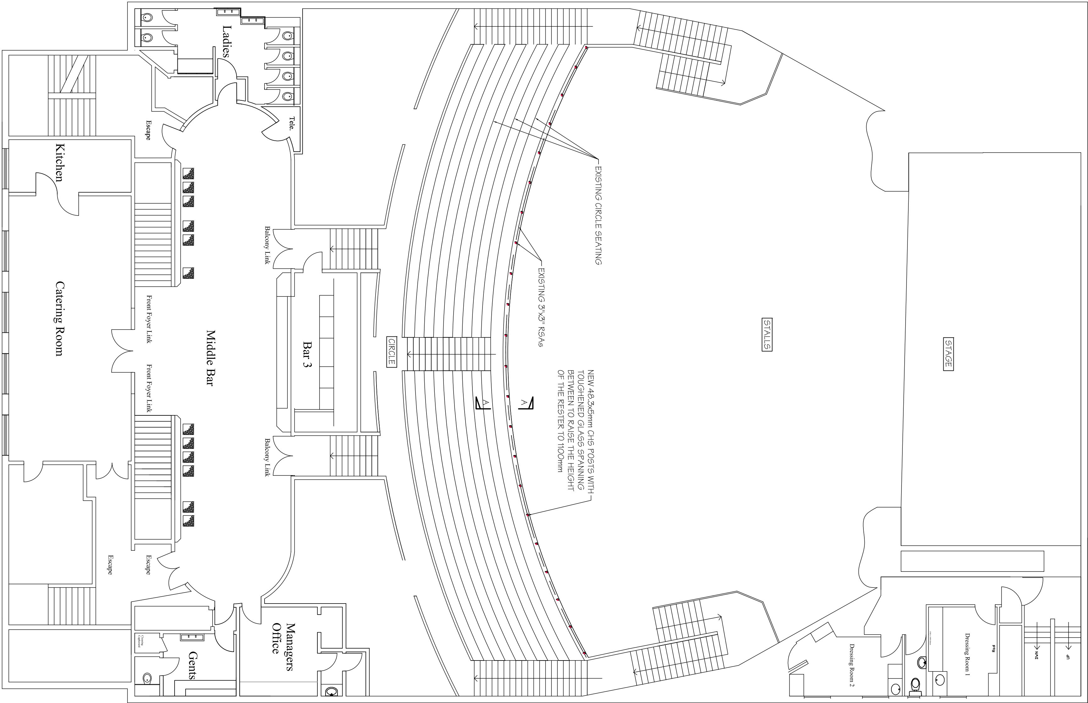
PROPOSED CIRCLE PLAN (SCALE 1:100 AT A1)
