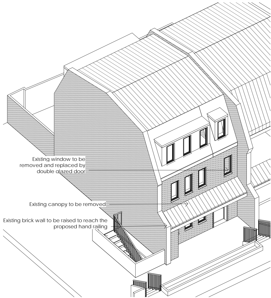
1 Existing 3D Front View
