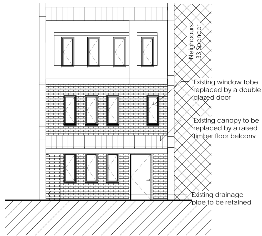
1 Existing Front Elevation
