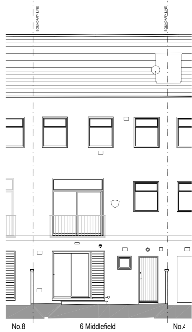
Existing Rear Elevation - 1:100 @ A3
