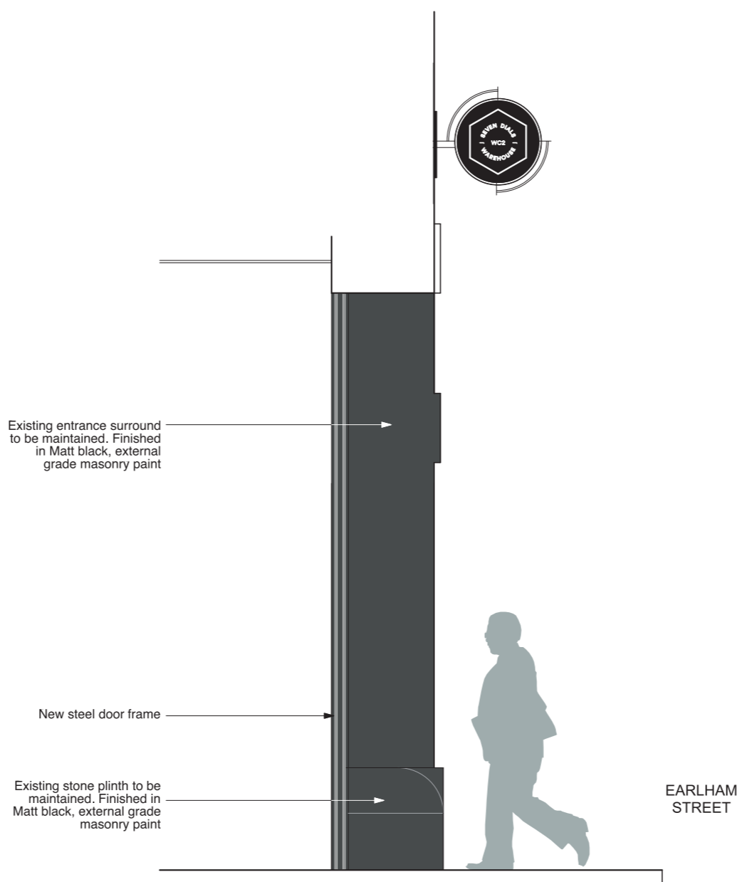
SECTION B - SEVEN DIALS WAREHOUSE
