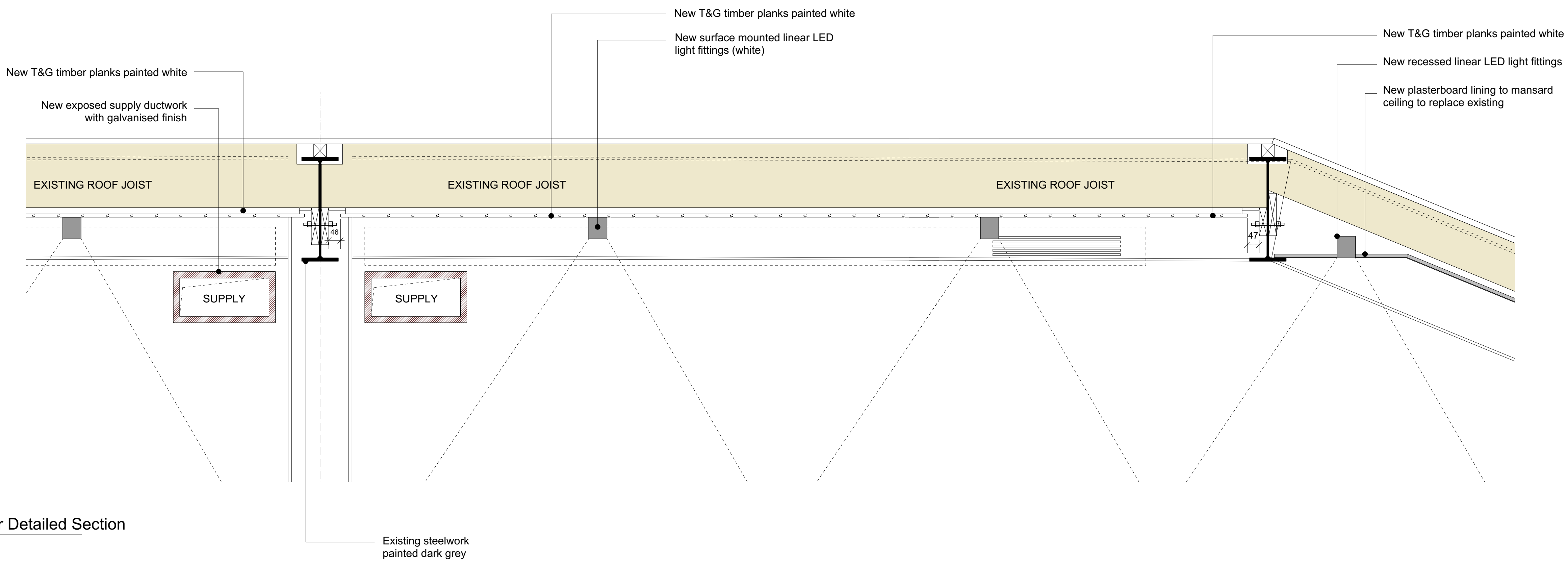
01 Proposed Third Floor Section AA Scale 1:25@A1
