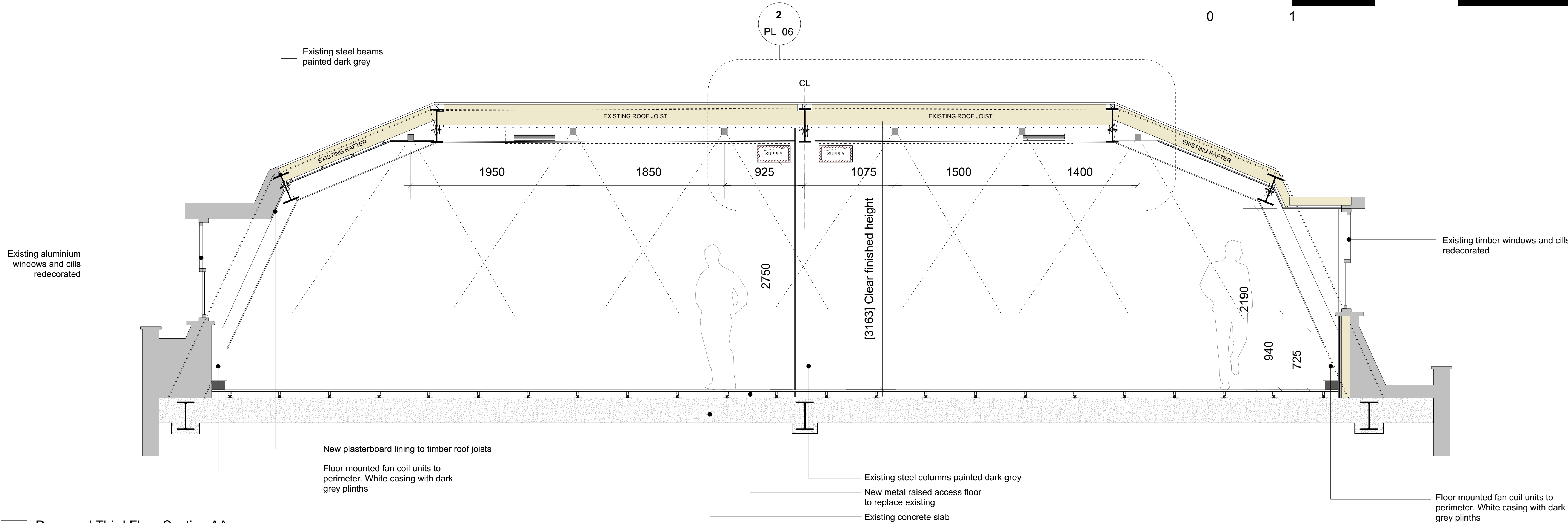
01 Proposed Third Floor Section AA Scale 1:25@A1
