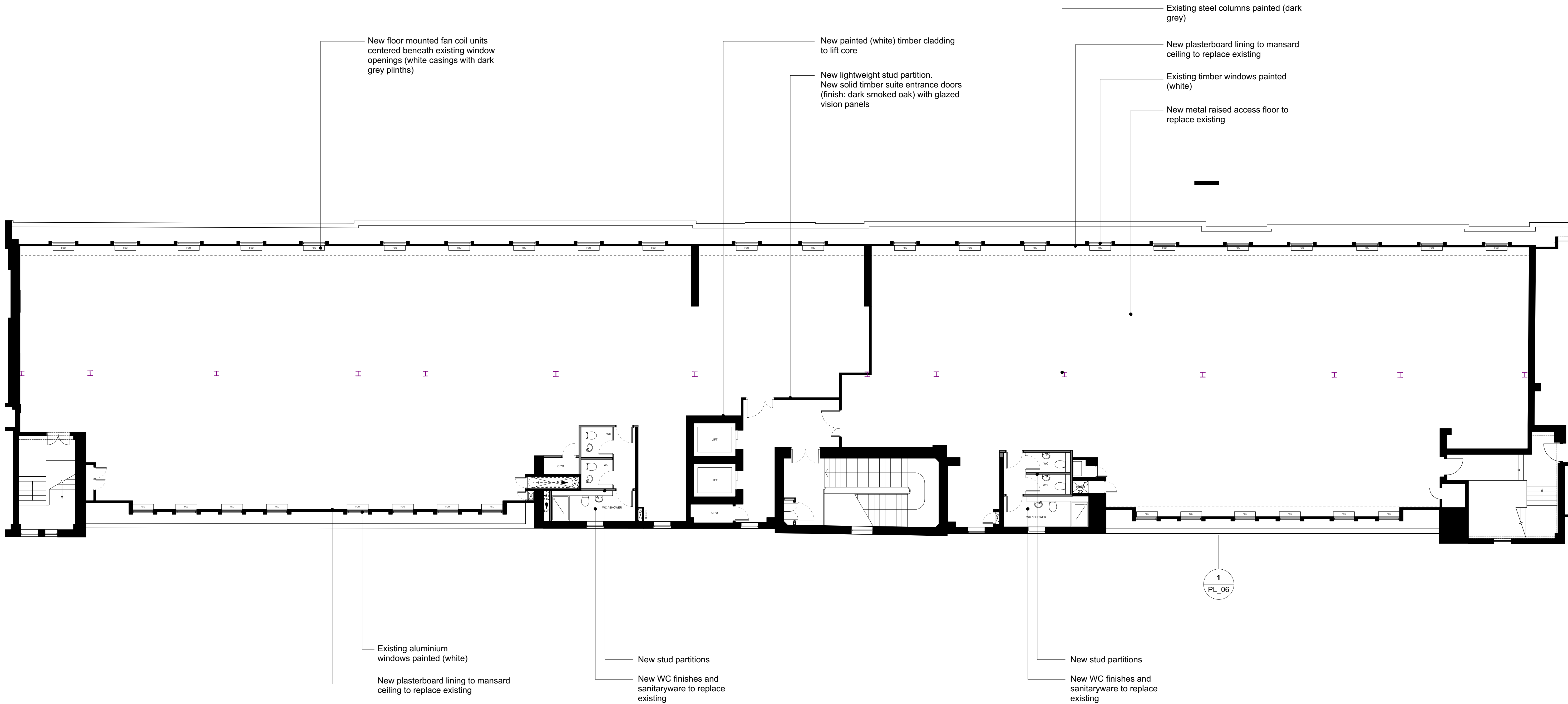
01 Proposed Third Floor Plan Scale 1:100@A1
