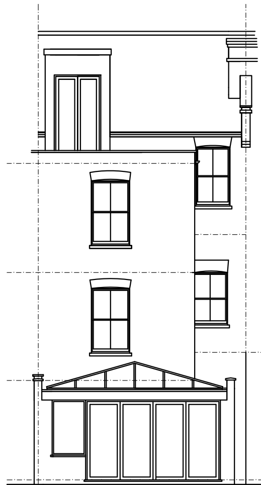
rear elevation
