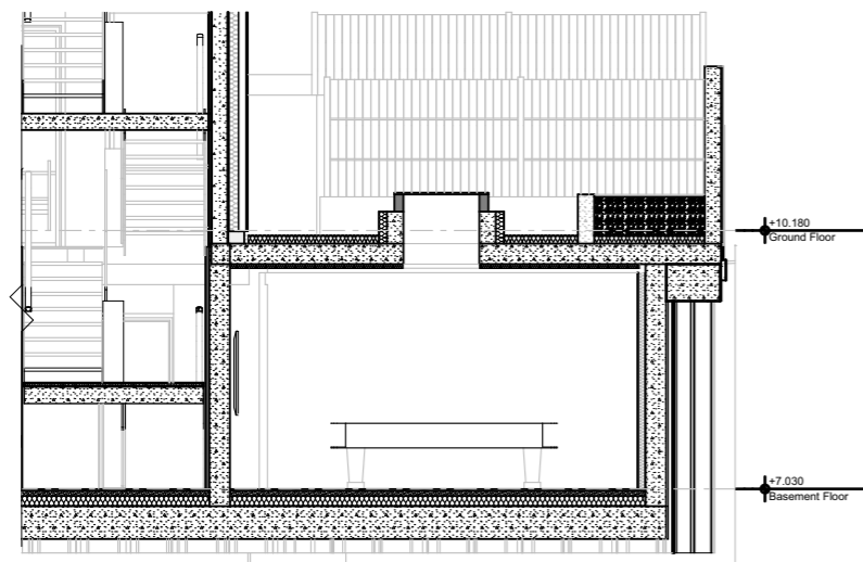
Section AA Scale @A3 - 1:100
