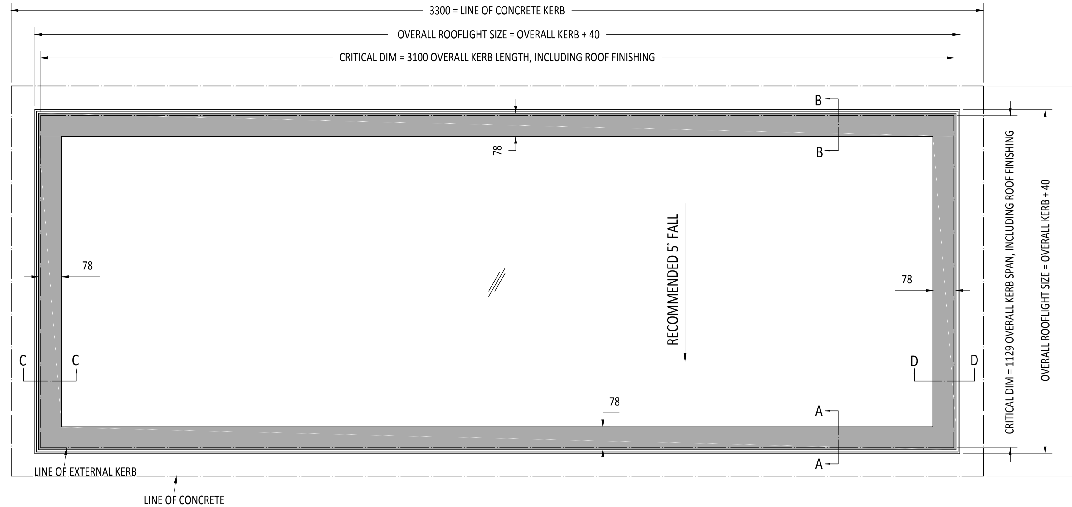
PLAN VIEW True view on slope
