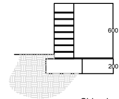
Side elevation of the wall on the boundary between the property and the pedestrian path.
