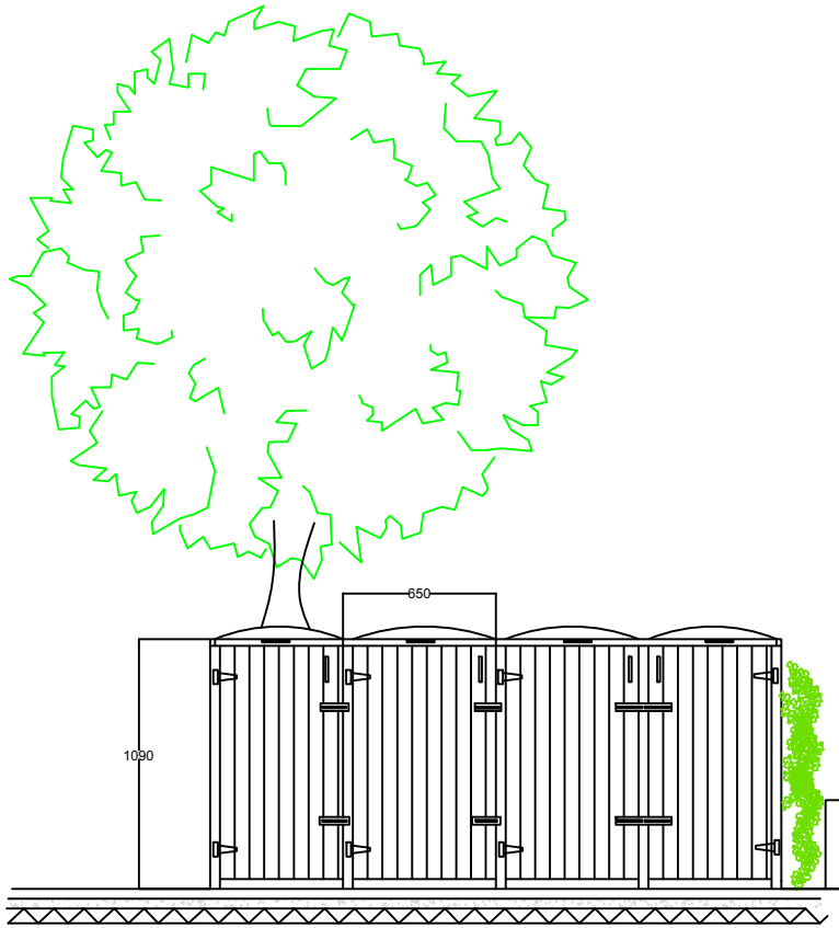
Bin Store Front and side elevation
