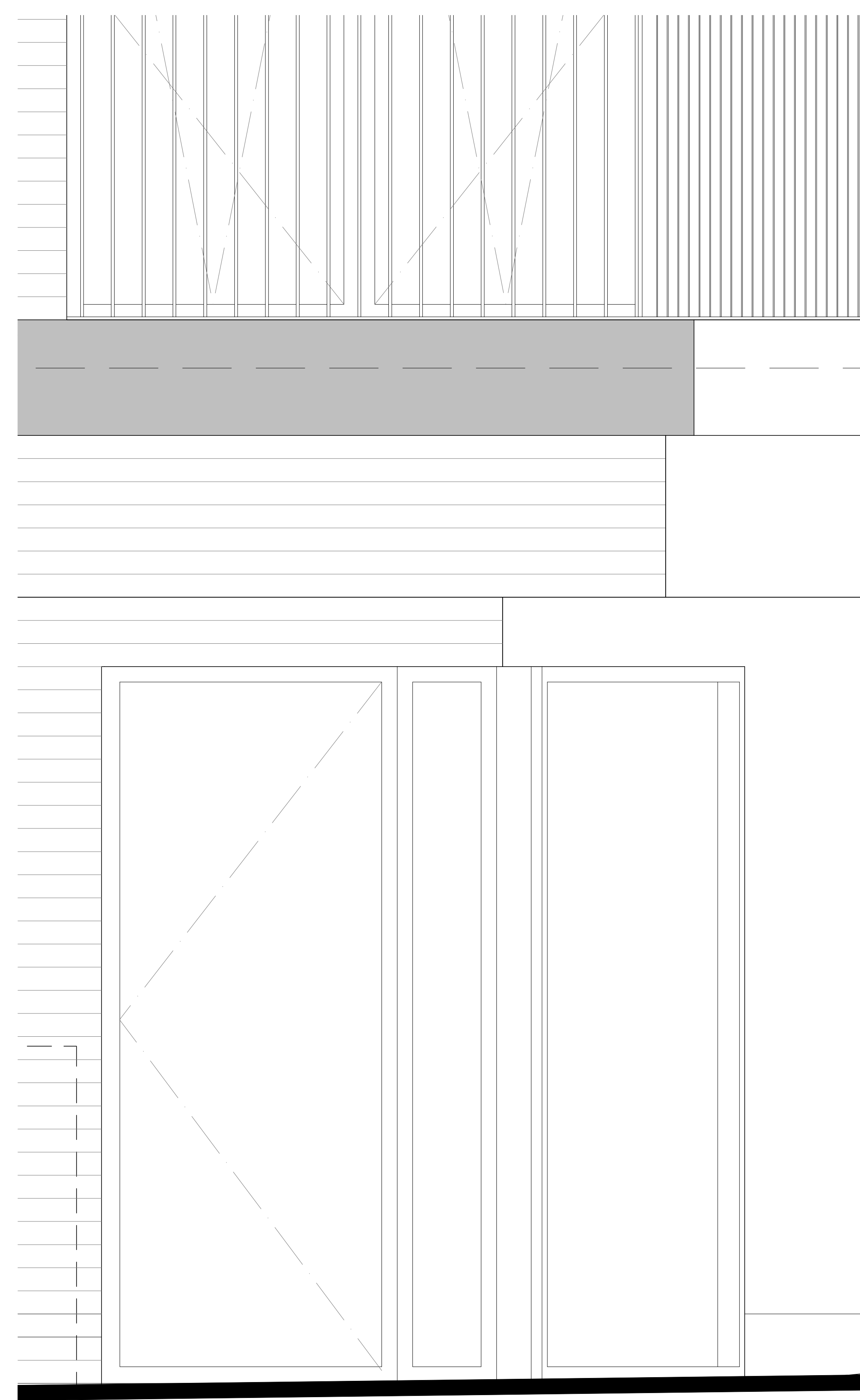
02 Malden Road Elevation 1:10
