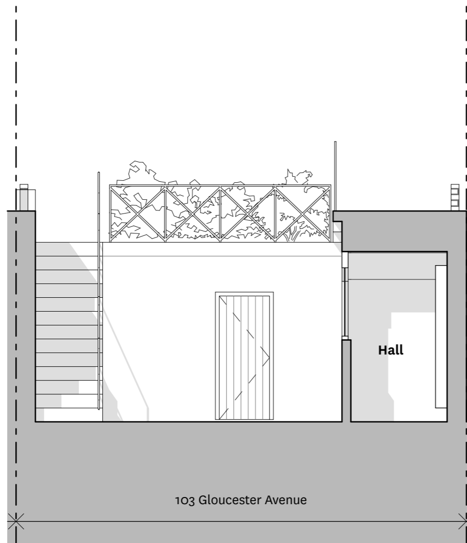
Existing Coal Store Elevation 1:50 @ A3
