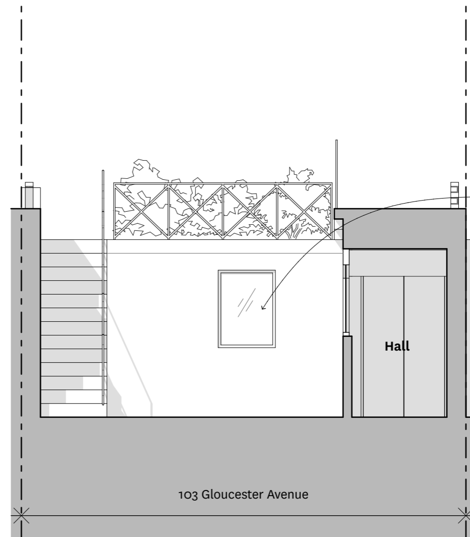
Proposed Coal Store Elevation 1:50 @ A3
