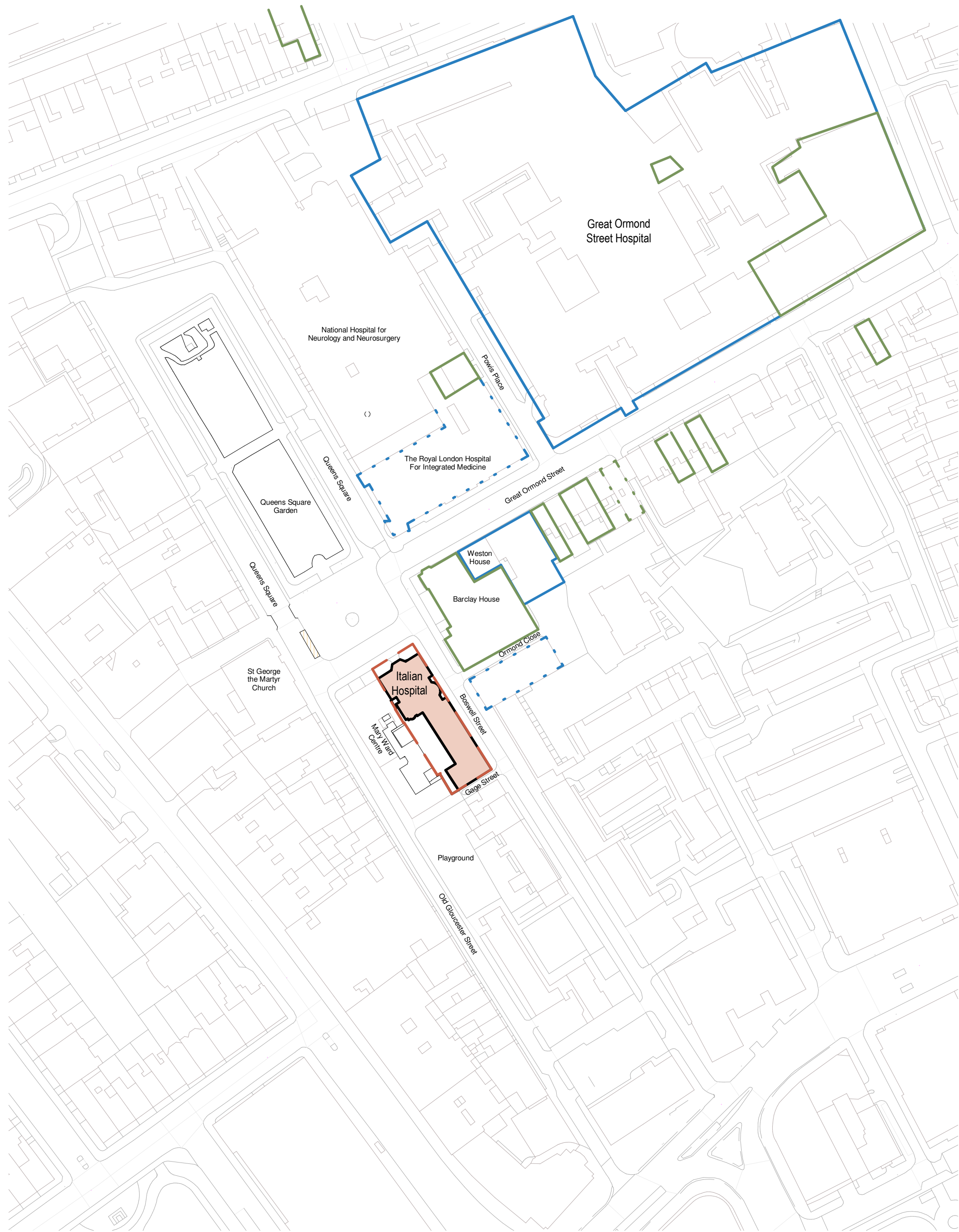
1 Location Plan 1 : 1250
